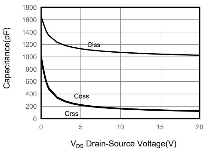
Figure 5. Capacitance
