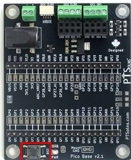
Figure 7: Reset button “RST” on the Pico Base.
