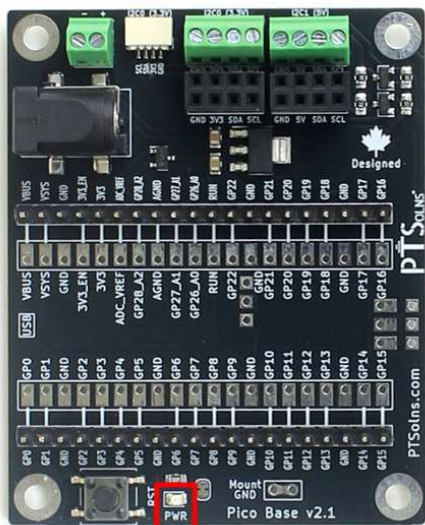
Figure 8: Power LED PWR on the Pico Base.
