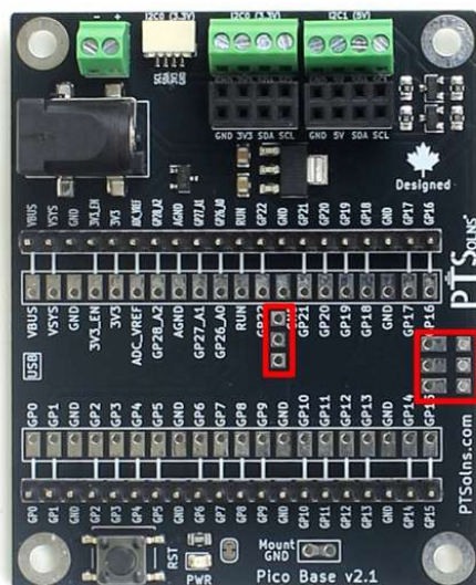
Figure 6: Debugging pins available on the Pico Base.
