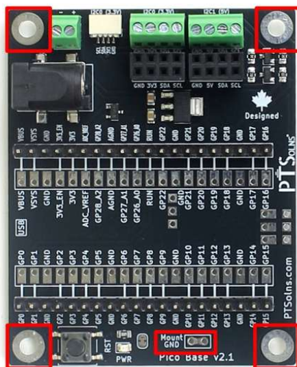
Figure 9: Mounting holes on the Pico Base.
