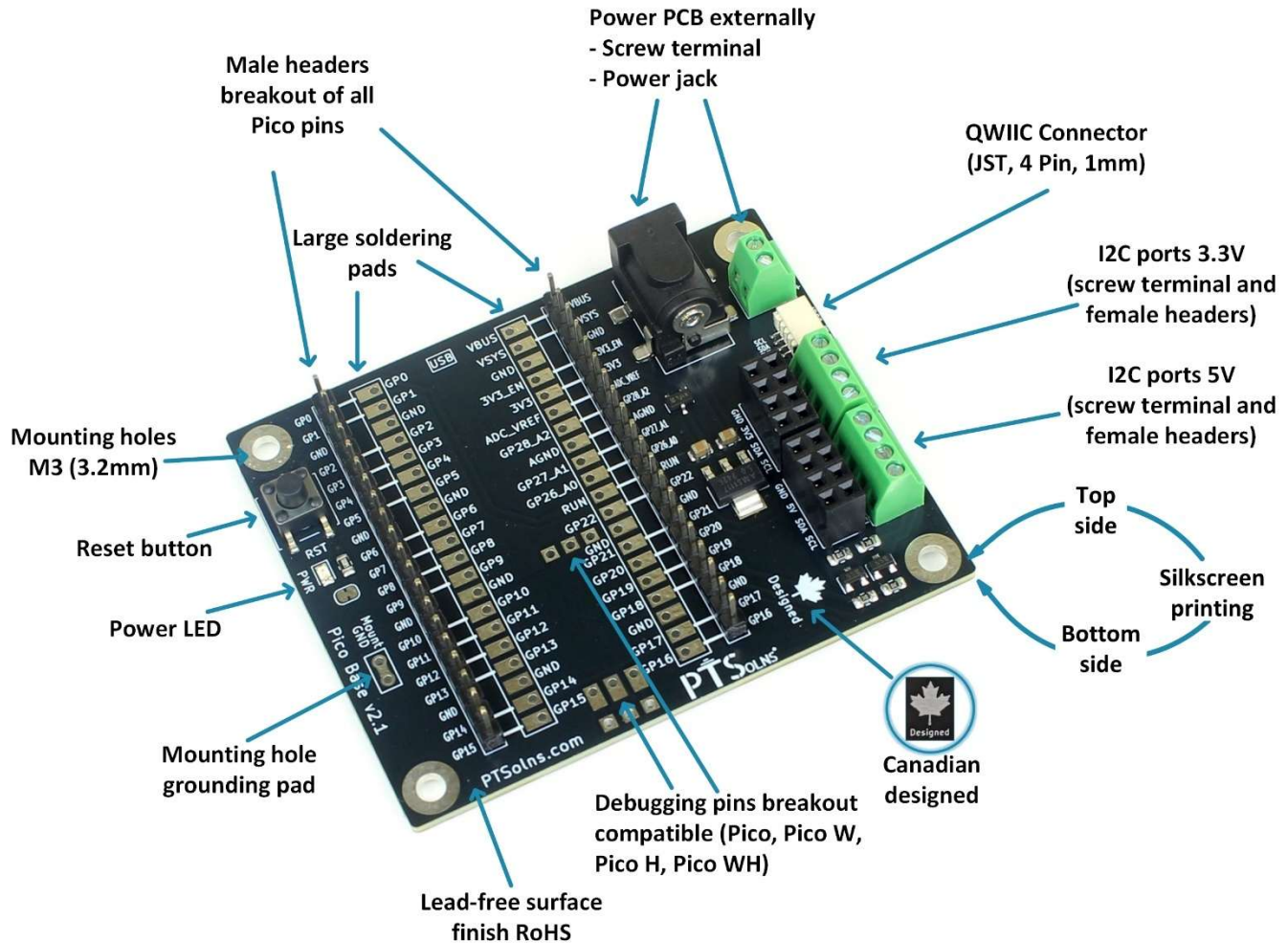
Figure 1: Features of the Pico Base.
