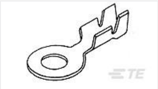
TE Part #60007-2 RING TERMINAL CRIMP TAB 26-22 AWG TPBR
