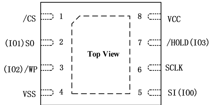
Figure 3.2. Pin Configuration DFN 4X3mm
