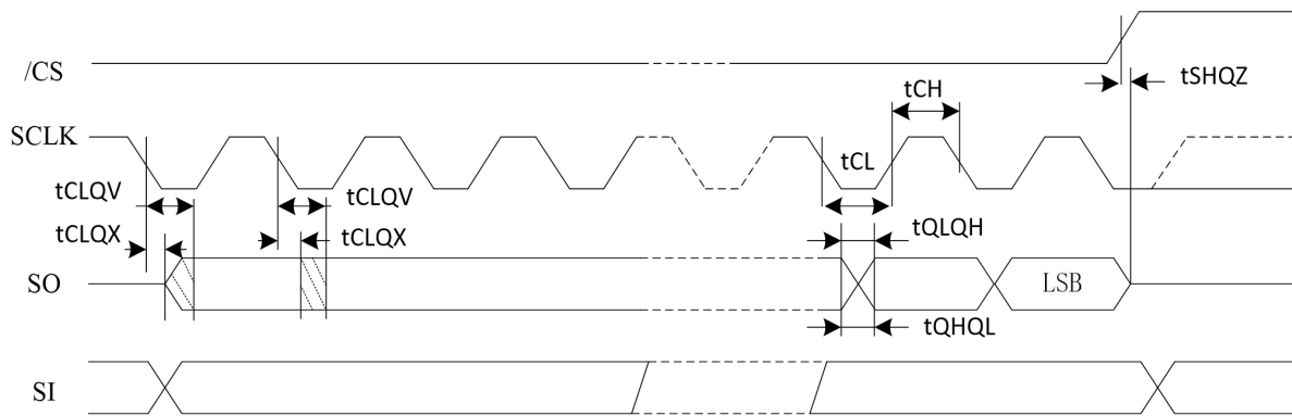
Figure 47. Output Timing
