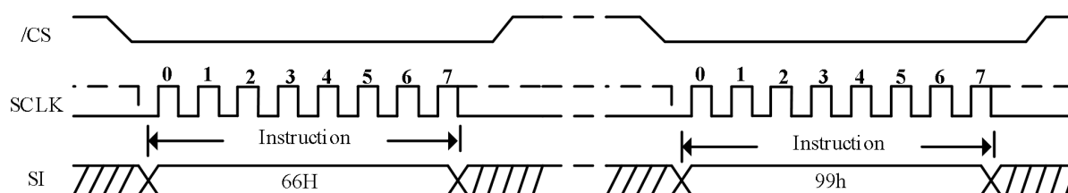
Figure 32. Enable Reset (66h) and Reset (99h) Command Sequence
