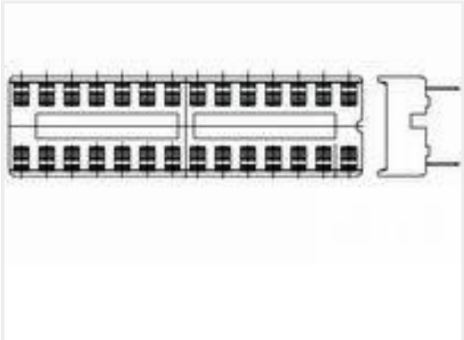
TE Part #1-2199298-2 8P,DIP SKT,300 CL,LDR,PB FREE
