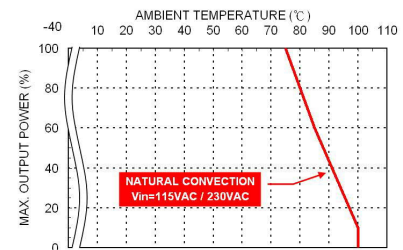
Derating Curve vs. Ambient Temperature MSC15USxxD xx=24/28/36/48/53 Connector Option : (-M / -T / -D)
