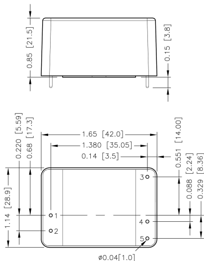
BOTTOM VIEW
