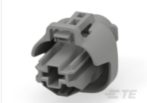
TE Part # 1544601-3 RECEPTACLE HOUSING, 8MM NG1, 1 WAY
