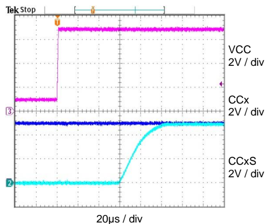
CC OVP Recovery
