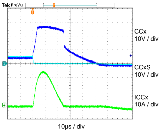
CC +80V Surge Event
