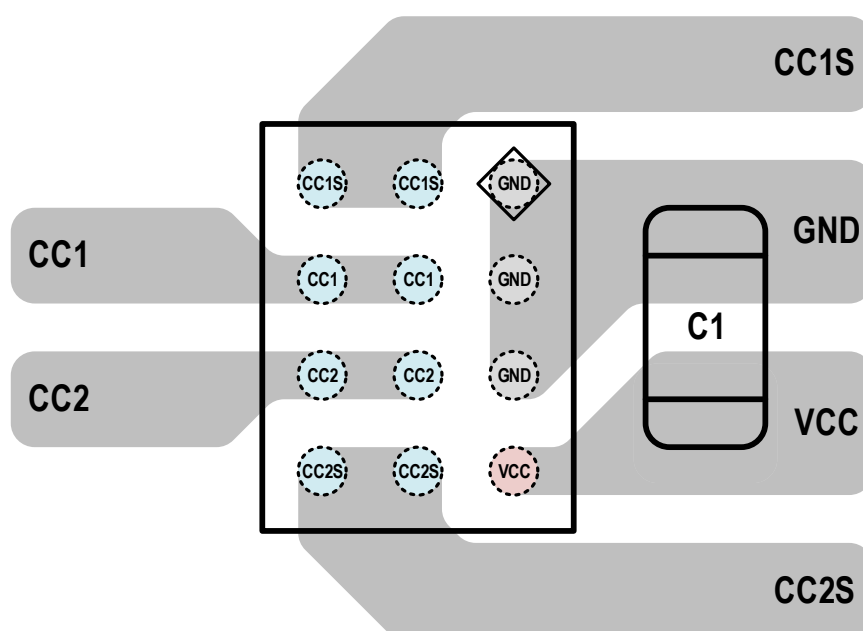
Figure 3. Recommended Layout
