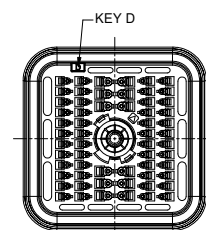
60 Position - Plug - Keyed D ARB16-60SDR-L018
