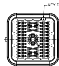
60 Position - Receptacle - Keyed D ARB12-60PDR-L018
