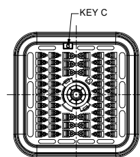
60 Position - Plug - Keyed C ARB16-60SCR-L018
