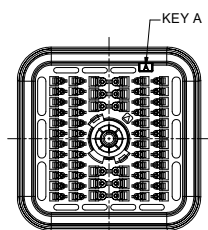
60 Position - Plug - Keyed A ARB16-60SAR-L018
