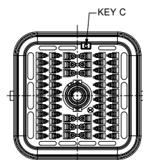
60 Position - Receptacle - Keyed C ARB12-60PCR-L018
