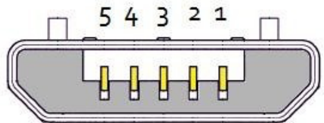
USB Micro-B
