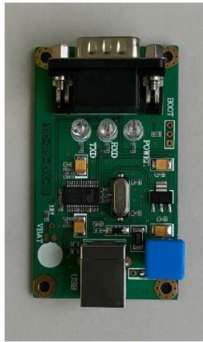
Adaptor Board
