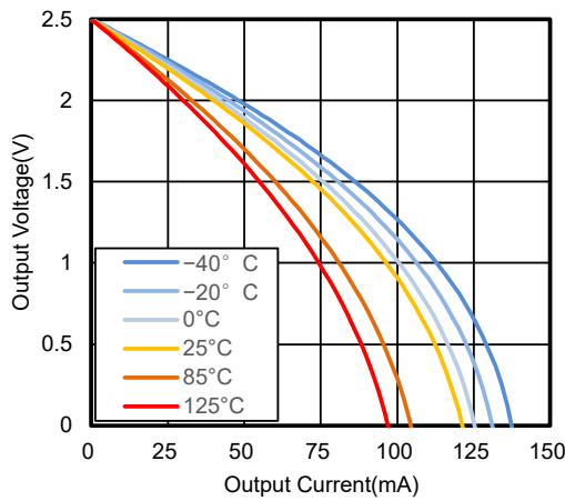
Figure 13. Output Voltage vs. Output Current, ( -V_S ) = -2.5 V, ( +V_S ) = 2.5 V
