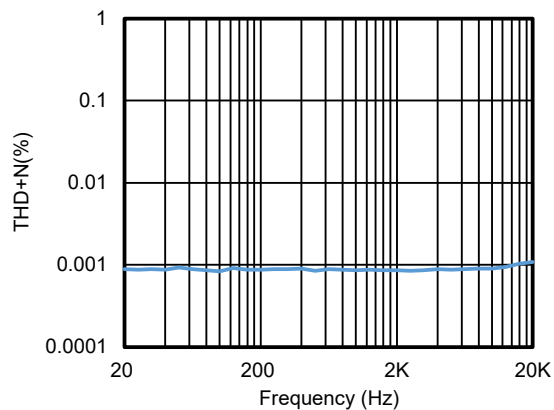
Figure 23. THD vs. Frequency, G = 1 , V_{IN} = 1\text{ V}_{RMS}
