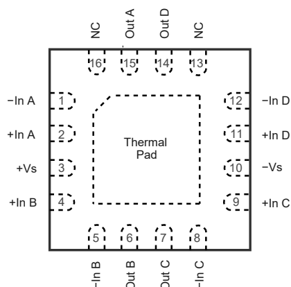
TPA6584V QFN3x3-16 Top View
