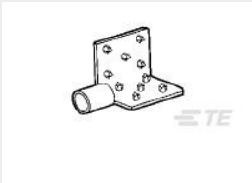
TE Part #2-329254-4 TERMINAL,TERMI-FOIL 12-10
