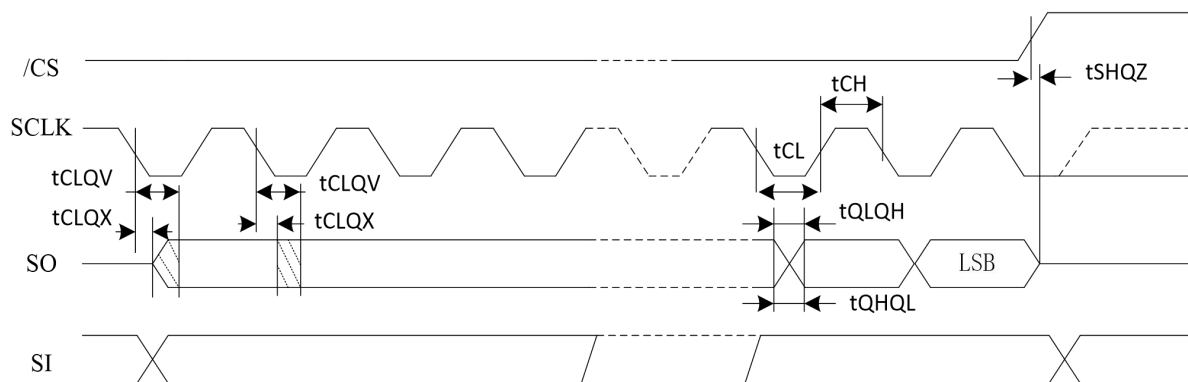
Figure 24. Output Timing
