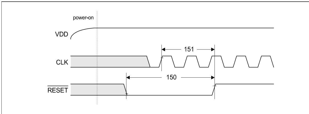
Figure 7-10 Reset Timing
