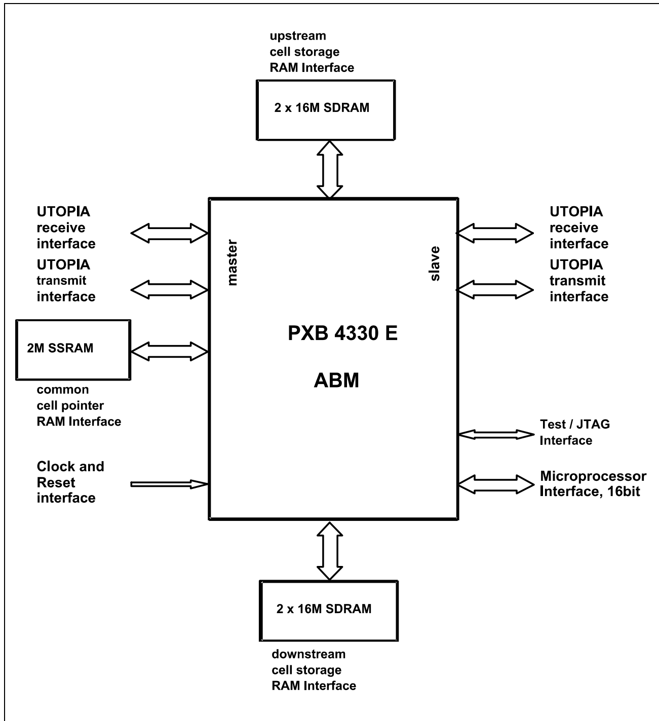
Figure 1-2 Logic Symbol
