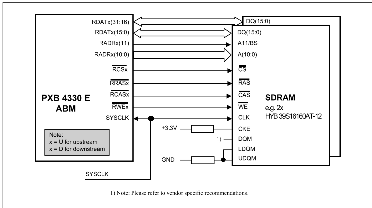
Figure 5-4 SDRAM Interfaces
