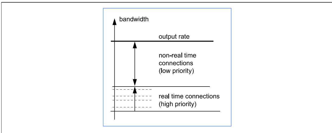
Figure 3-4 Scheduler Behavior
