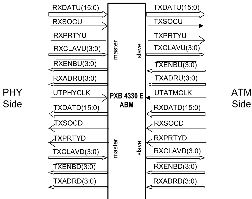
Figure 5-1 UTOPIA Interfaces
