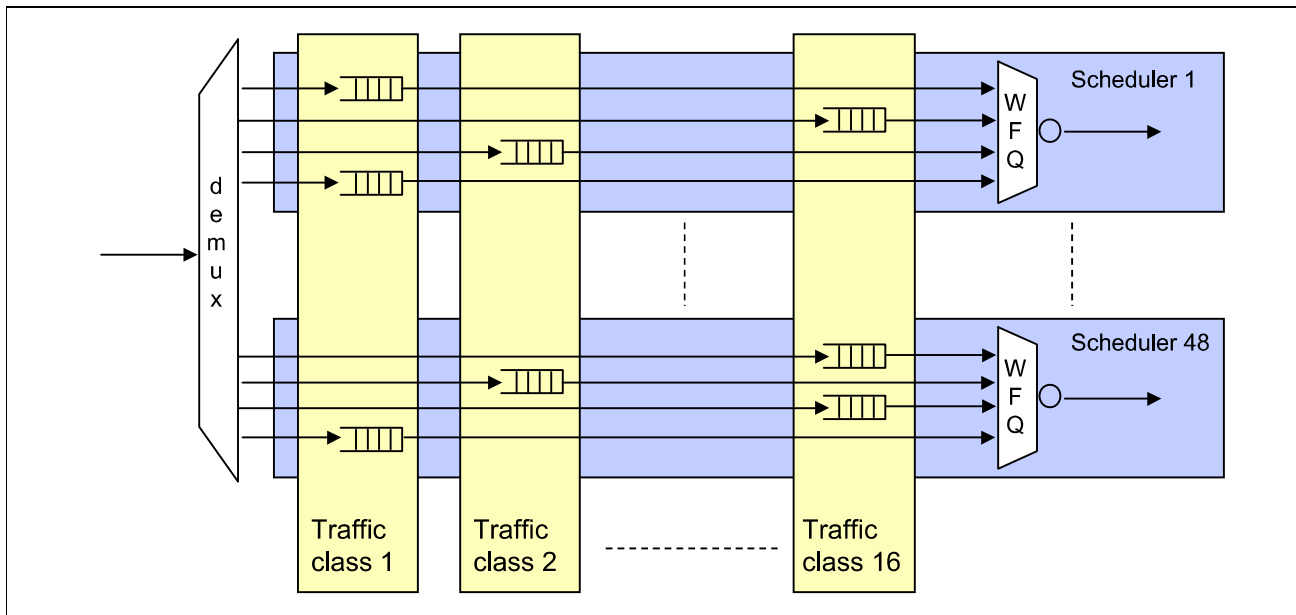
Figure 3-9 Queue Grouping
