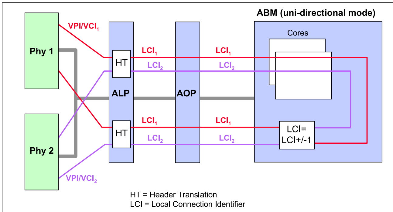
Figure 1-10 Connection Identifiers in Mini-Switch Configuration
