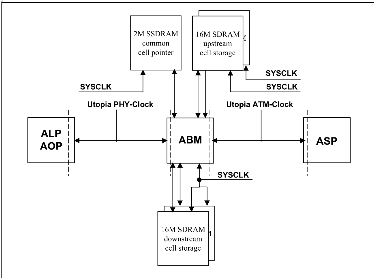
Figure 5-8 Clock Concept
