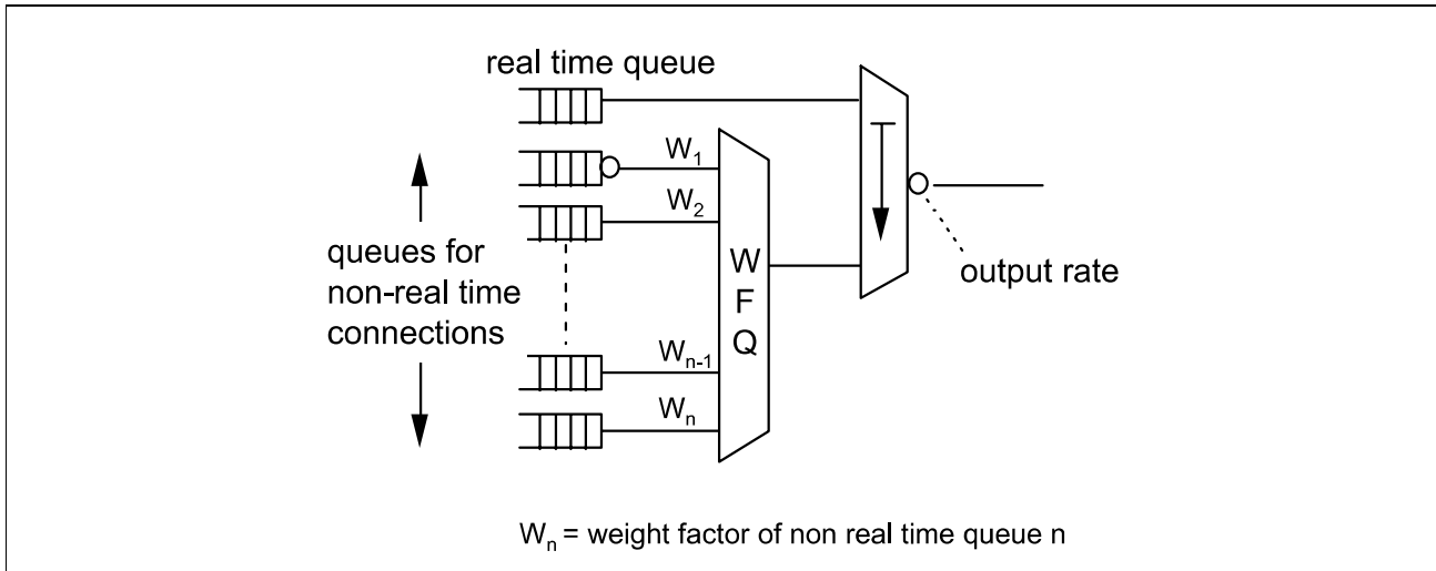
Figure 3-3 Scheduler Structure
