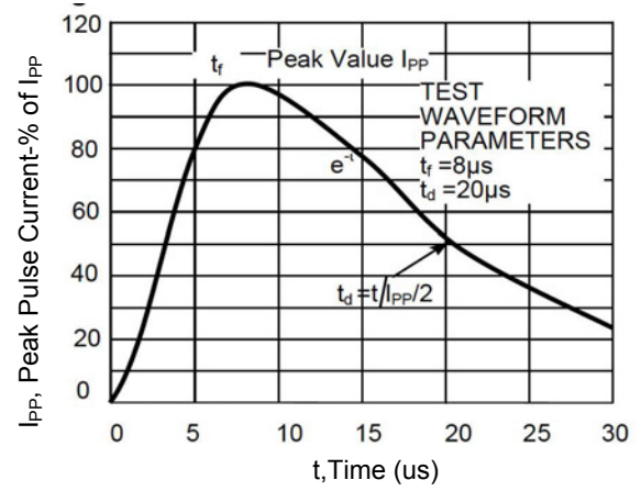
Figure 2. Pulse Waveform
