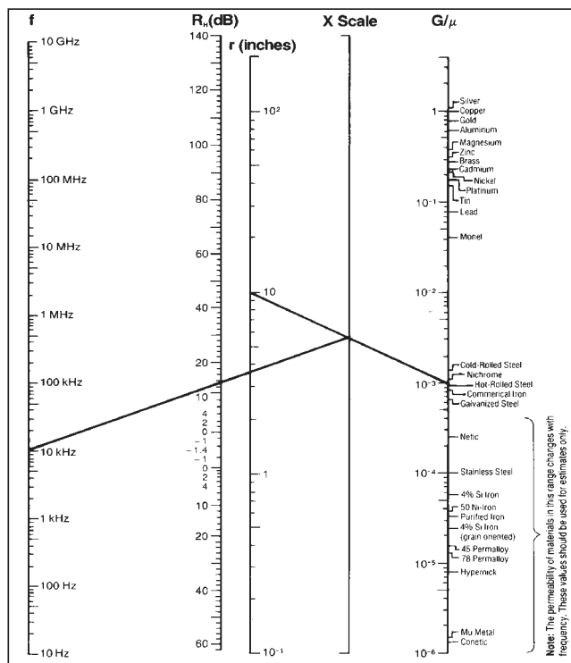
Figure 10-6 Magnetic Field Reflection Loss Nomograph, RH 1
