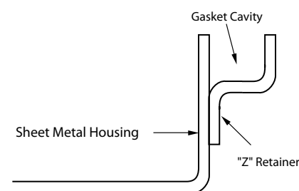
Figure 1-3. Z-Retainer Forms Gasket Cavity
