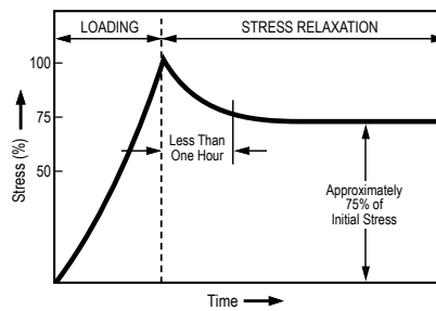
Graph 3-15. Stress Relaxation
