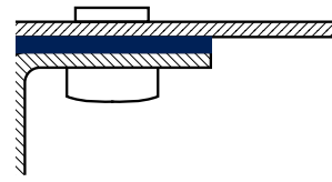
Figure 1-6. External Bolting Prevents EMI Leakage
