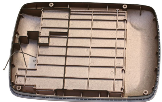
Plastic electronics housing painted with electrically conductive copper-filled coating
