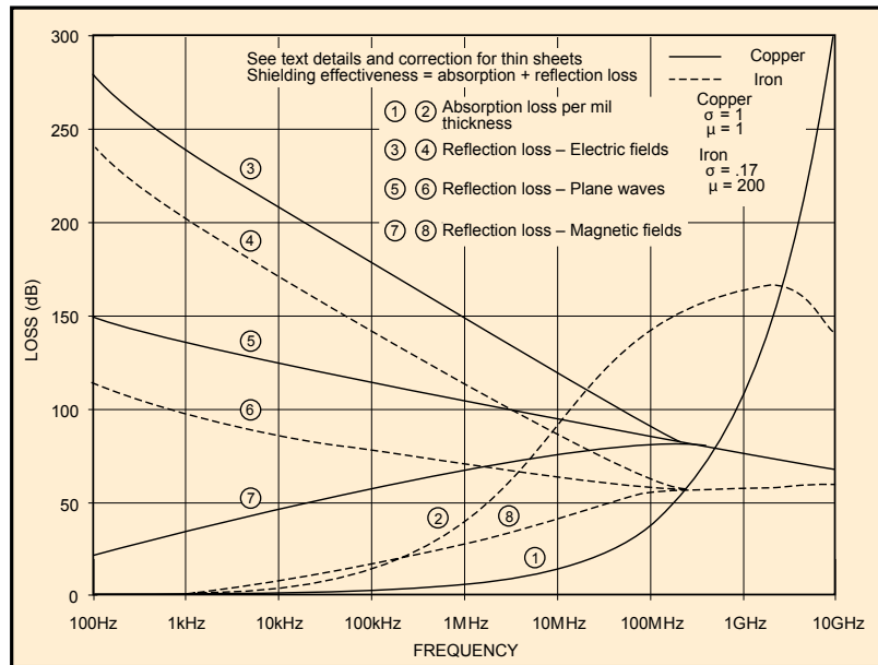
Graph 10-1 Shielding Effectiveness of Metal Barriers
