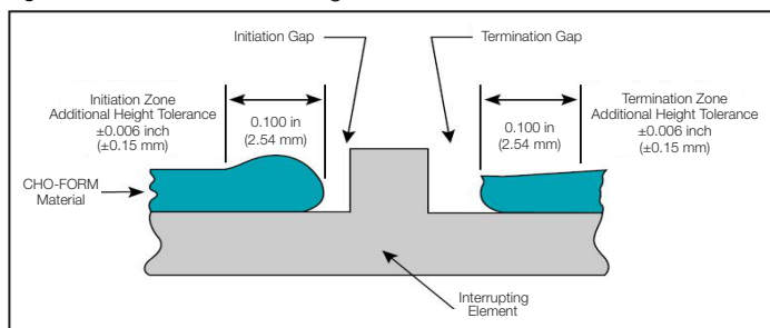
Figure 7-3 Side View Gasket height tolerances
