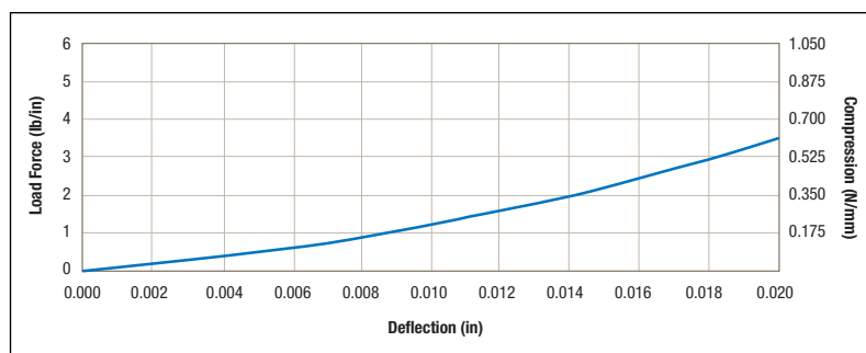
Graph 6-2 Typical Compression-Deflection Curve Predicted by FEA
