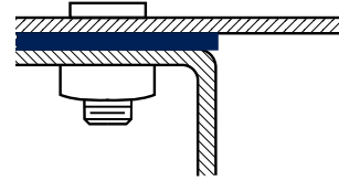
Figure 1-7. Insert Pressed-In and Flared Makes EMI Tight Joint (Alternate: Weld or Cement with Conductive Epoxy)
