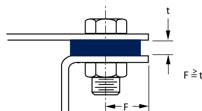
Figure 1-4. Flat Gasket on Sheet Metal Flange
