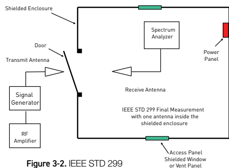
Figure 3-2. IEEE STD 299
