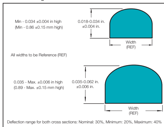
Figure 7-4 Suggested cross sections with height-to-width ratio of 0.85
