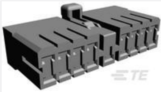
TE Part #172500-1 MIC MARK-2 PLUG HSG 17P
