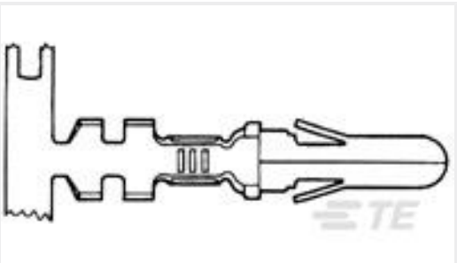
TE Part #350391-2 .140 DIA PIN 14-10 PTPPHBZ L/P
