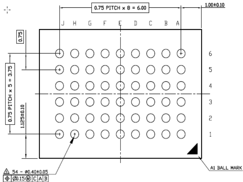
BOTTOM VIEW
