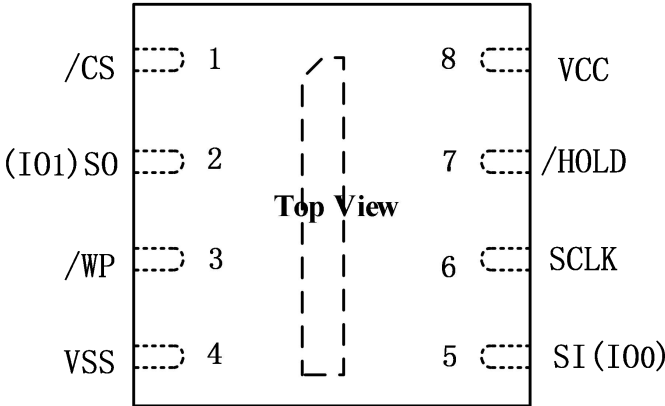
Figure 3. Pin Configuration USON8 2X3mm
