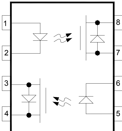
FIGURE 2. Terminal connections.
