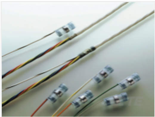
TE Part #D03269-000 B-155-07-35-22-5
