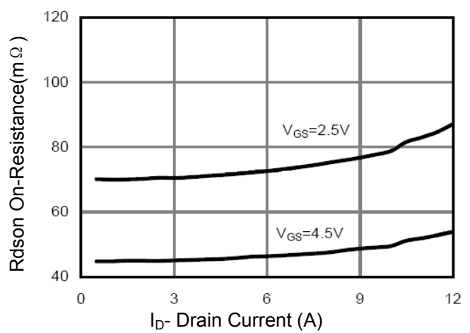
Figure 6 Drain-Source On-Resistance
