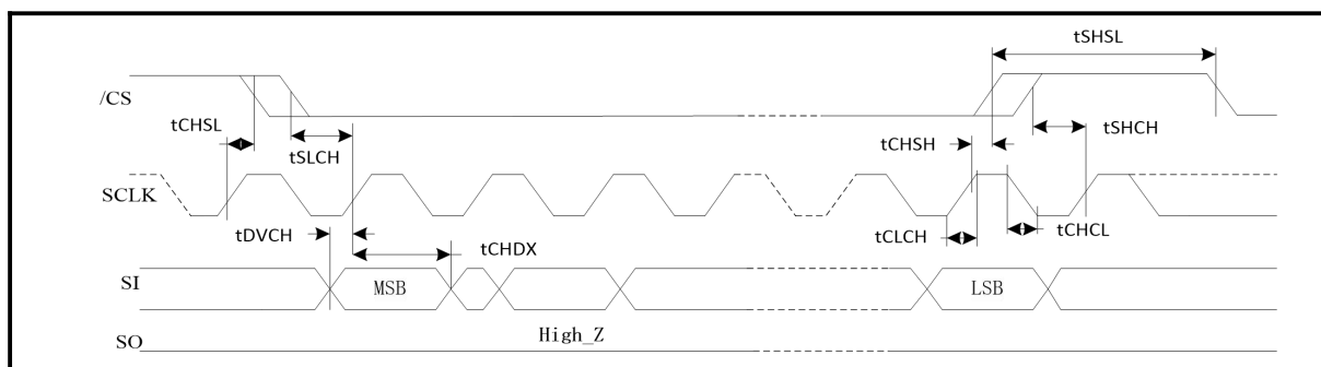
Figure 46. Output Timing
