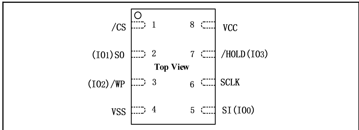
Figure 3. Pin Configuration USON8 2X3mm, USON8 4X3mm and WSON8 5X6mm
