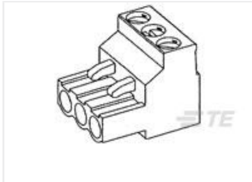
TE Part #796635-3 3 POS 5.08MM R/A PLUG,TRM BLK
