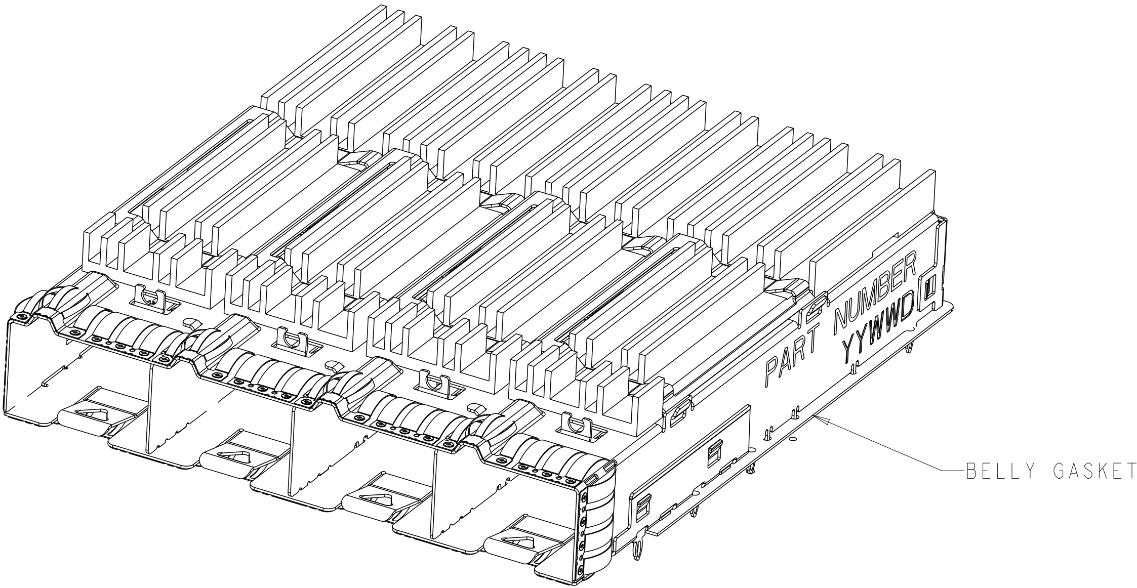
SCALE 3:1 1-2356208-2 AS SHOWN WITH BELLY GASKET AND WITHOUT LP UNSPECIFIED DIMENSIONS ARE SAME AS 2356208-1
