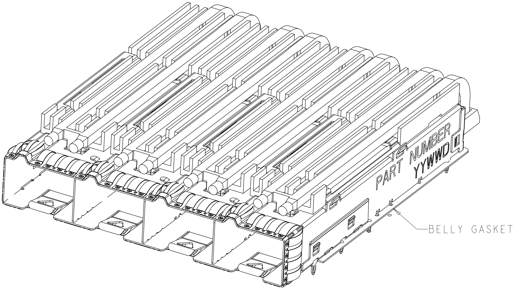
SCALE 3:1 2356208-6 AS SHOWN WITH BELLY GASKET UNSPECIFIED DIMENSIONS ARE SAME AS 2356208-1
