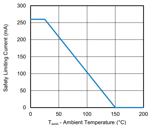
Fig. 23 - VIA0250DD Thermal Derating Curve, Dependence of Safety Limiting Values With Case Temperature per DIN VDE 0884-11
