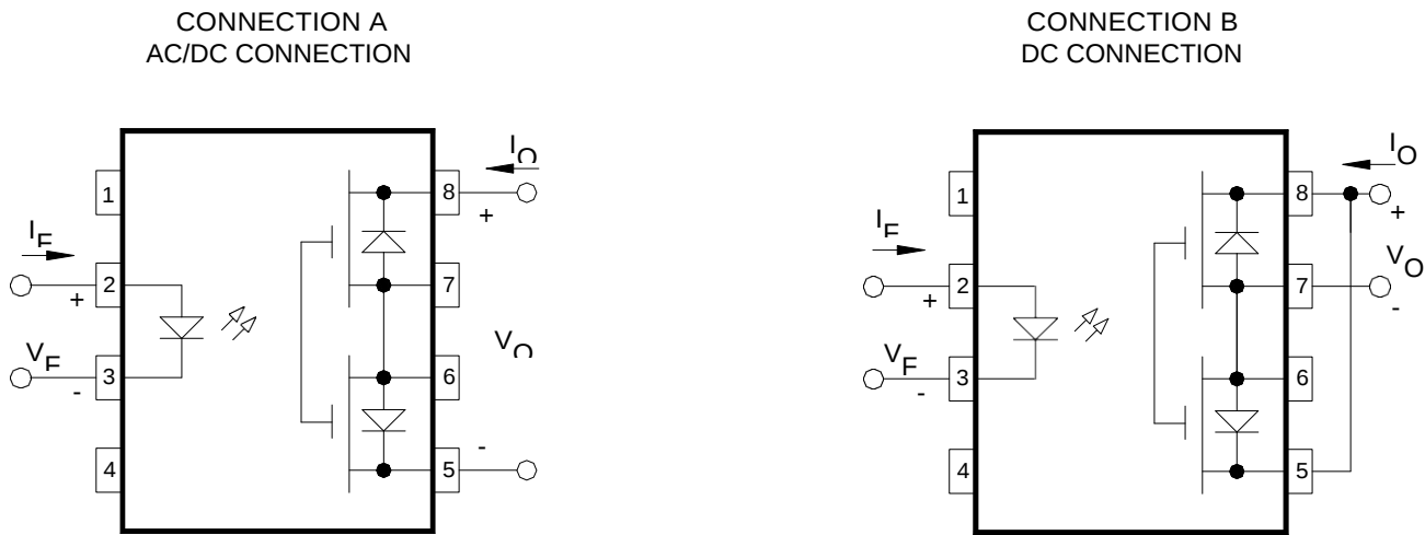
Figure 1 - Terminal Connections
