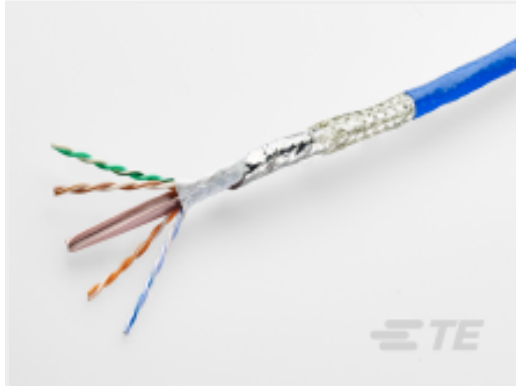
TE Part # EK3566-000 C6A-24B134XK18A
