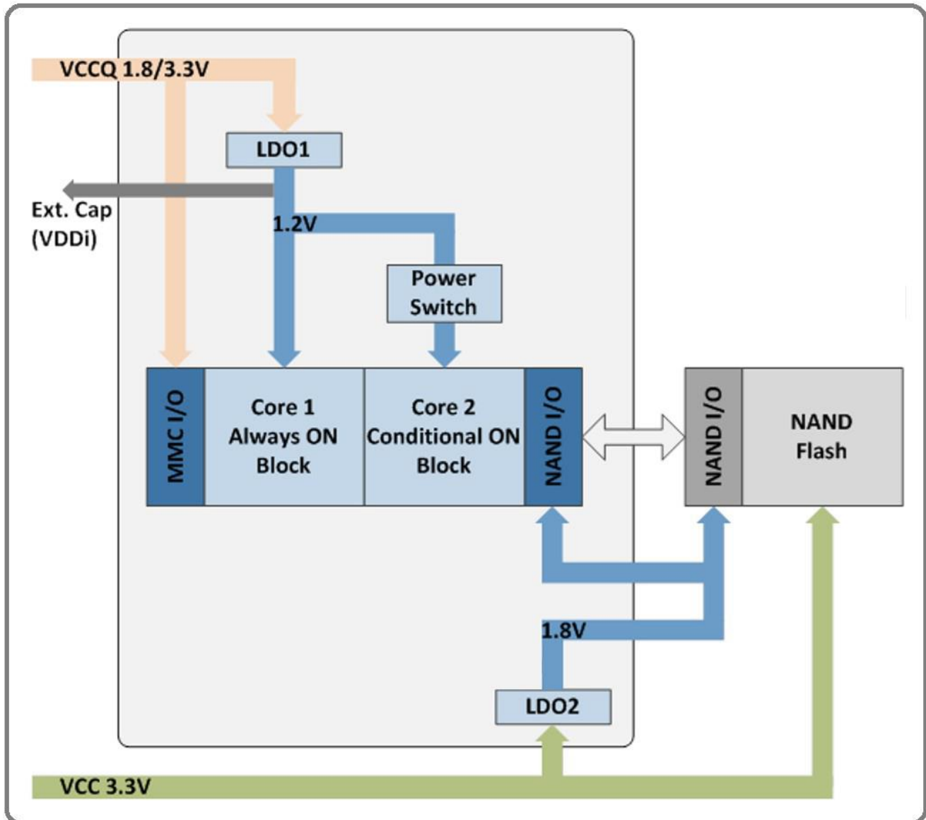
Figure 3. JSMC08AUM1ASAEA-SU Block Diagram
