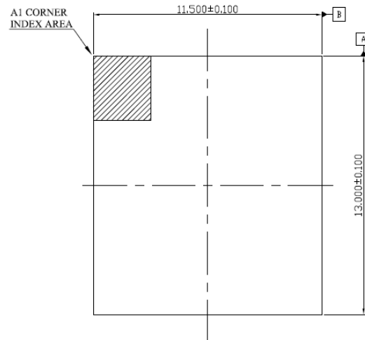
Figure 1. 11.5 x 13.0 x 1.0 (mm) Package Dimension
