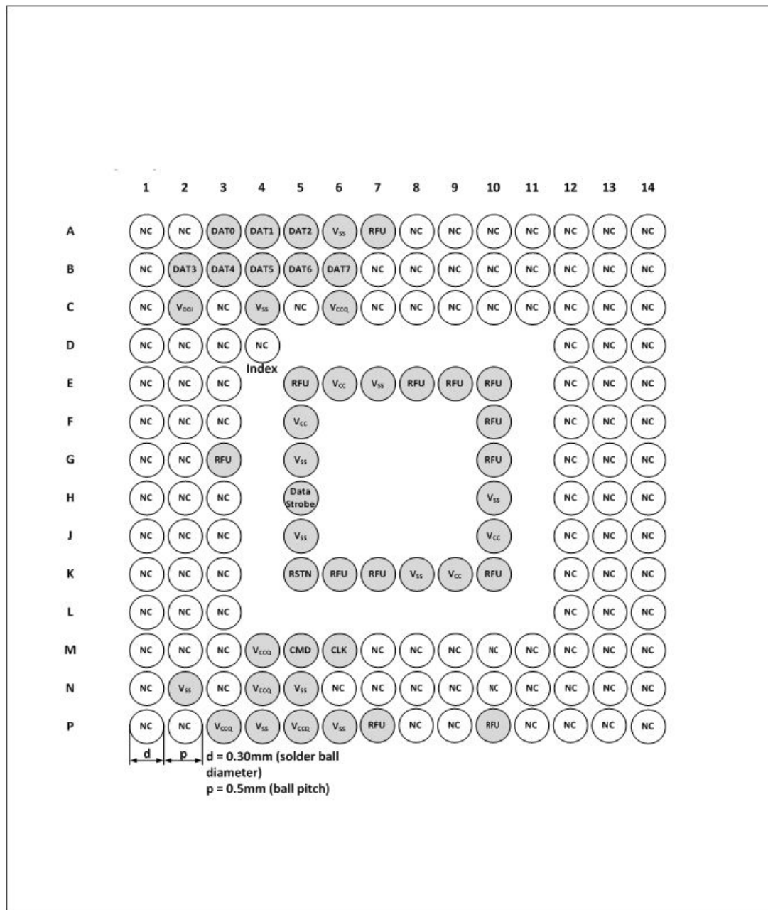
Figure 2. eMMC Package Ball Assignment
