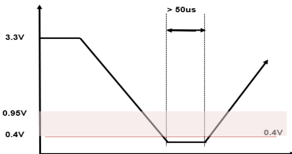
Figure Appendix 3. Recommended VCCQ power-off and Recovery Curve
