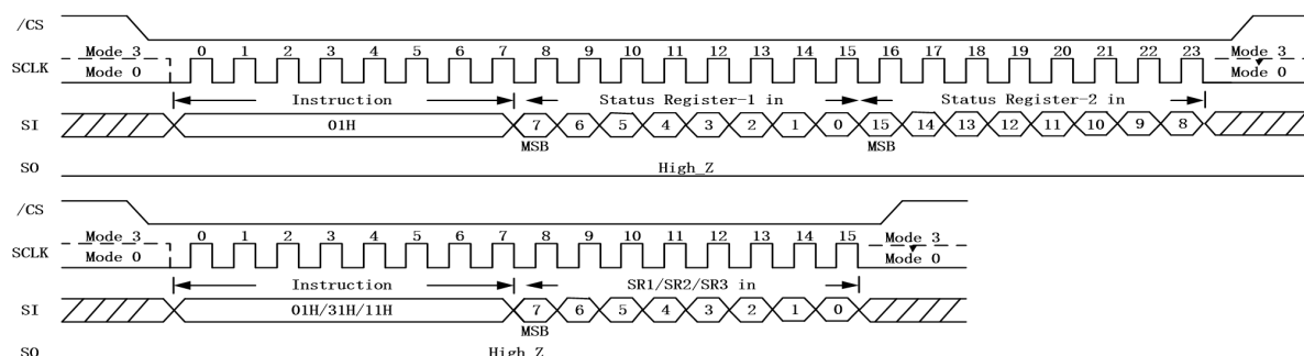
Figure 7.1.6. Write Status Register Instruction
