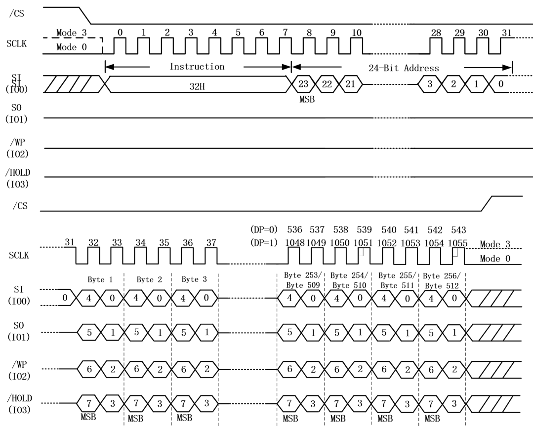
Figure 7.4.3. Quad Input Page Program Instruction
