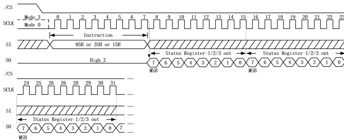
Figure 7.1.4. Read Status Register Instruction
