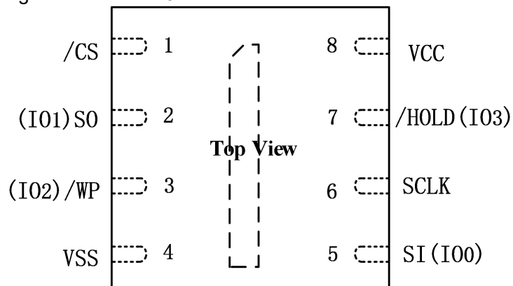
Figure 3.a. Pin Configuration DFN 2X3mm
