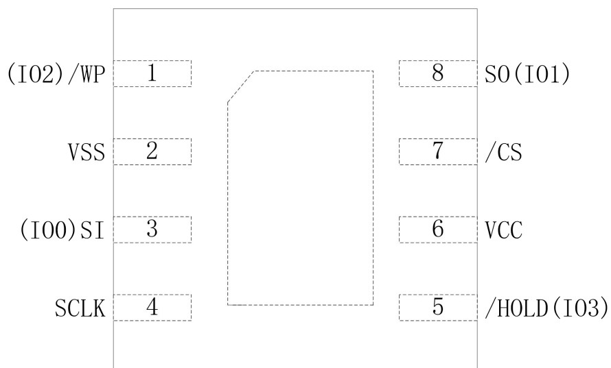
Figure 3.b. Pin Configuration DFN 1.5X1.5mm
