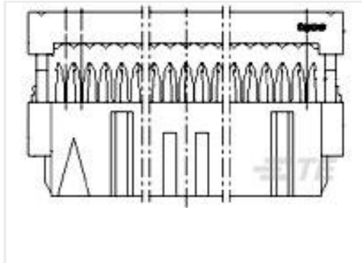
TE Part #4-215911-0 AMP LATCH, L.P.
