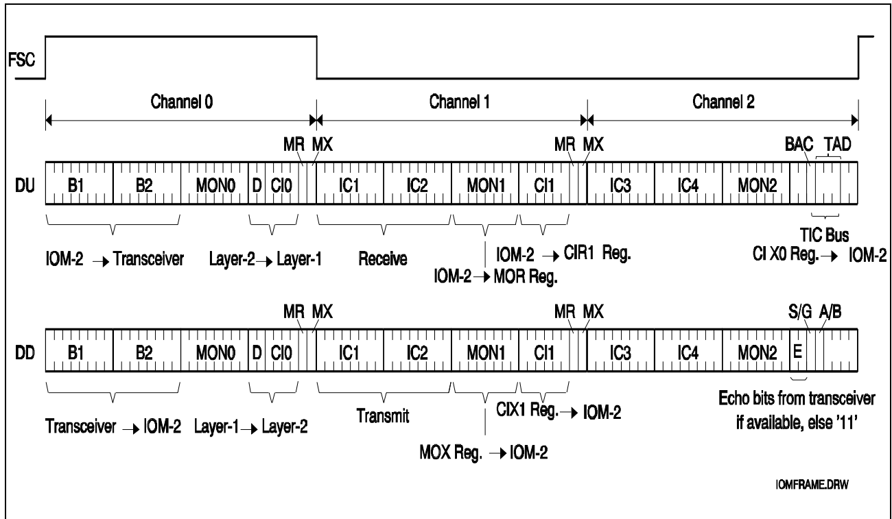
Figure 102 IOM-2 Frame Structure in Terminal Mode
