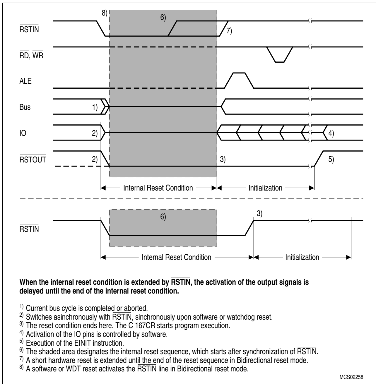
Figure 131 Reset Input and Output Signals
