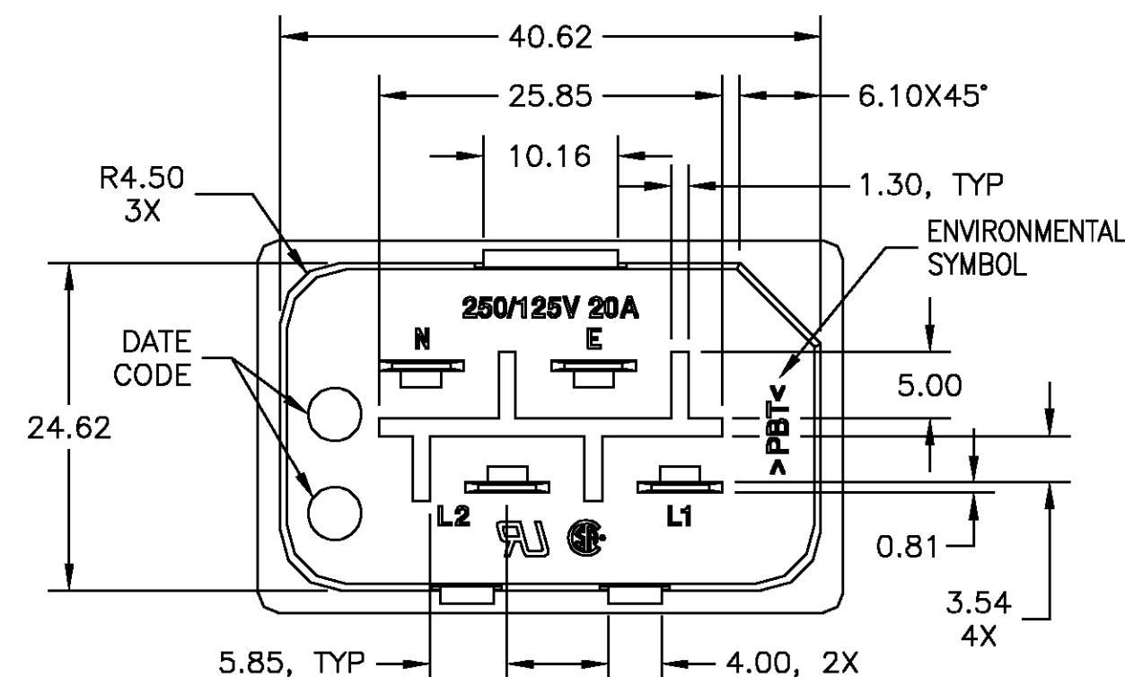
BOTTOM VIEW SHOWING MARKING
