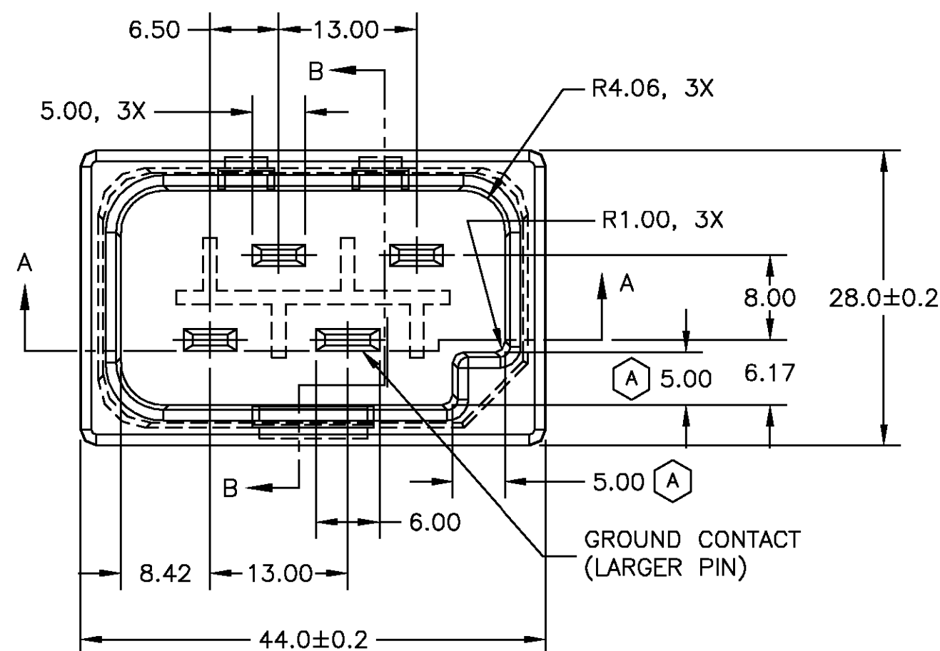
TOP VIEW
