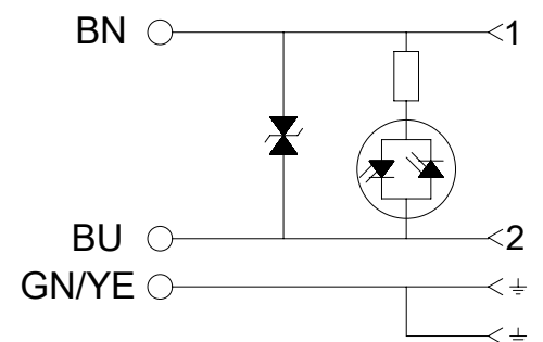
ELECTRICAL DIAGRAM S0
