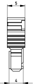
Cover pressed on
