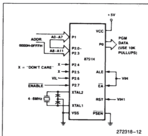
Figure 6. Program Verification
