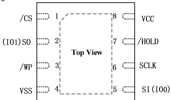
Figure 4. Pin Configuration USON8 3X3mm
