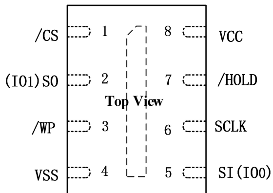
Figure 3. Pin Configuration USON8 2X3mm
