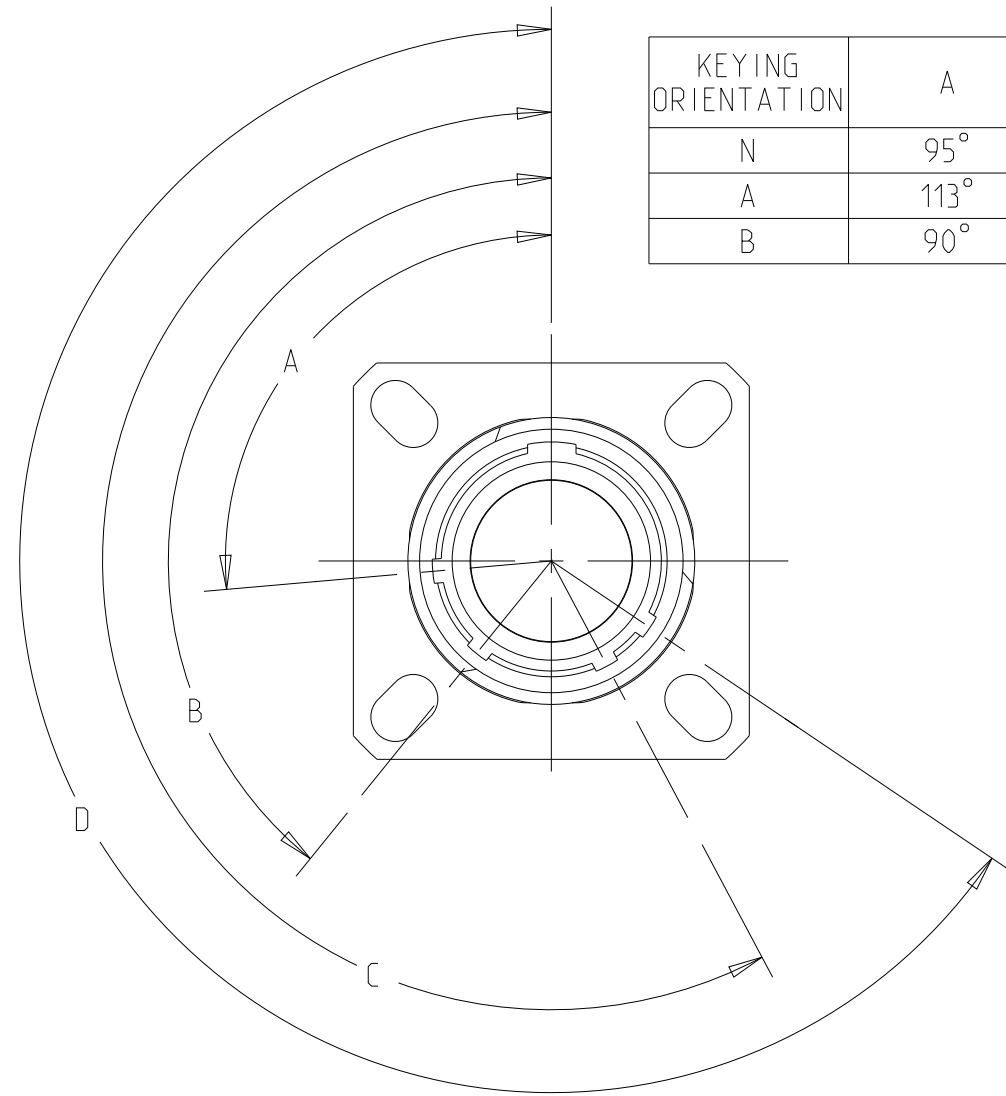
KEYING ORIENTATION DETAIL
