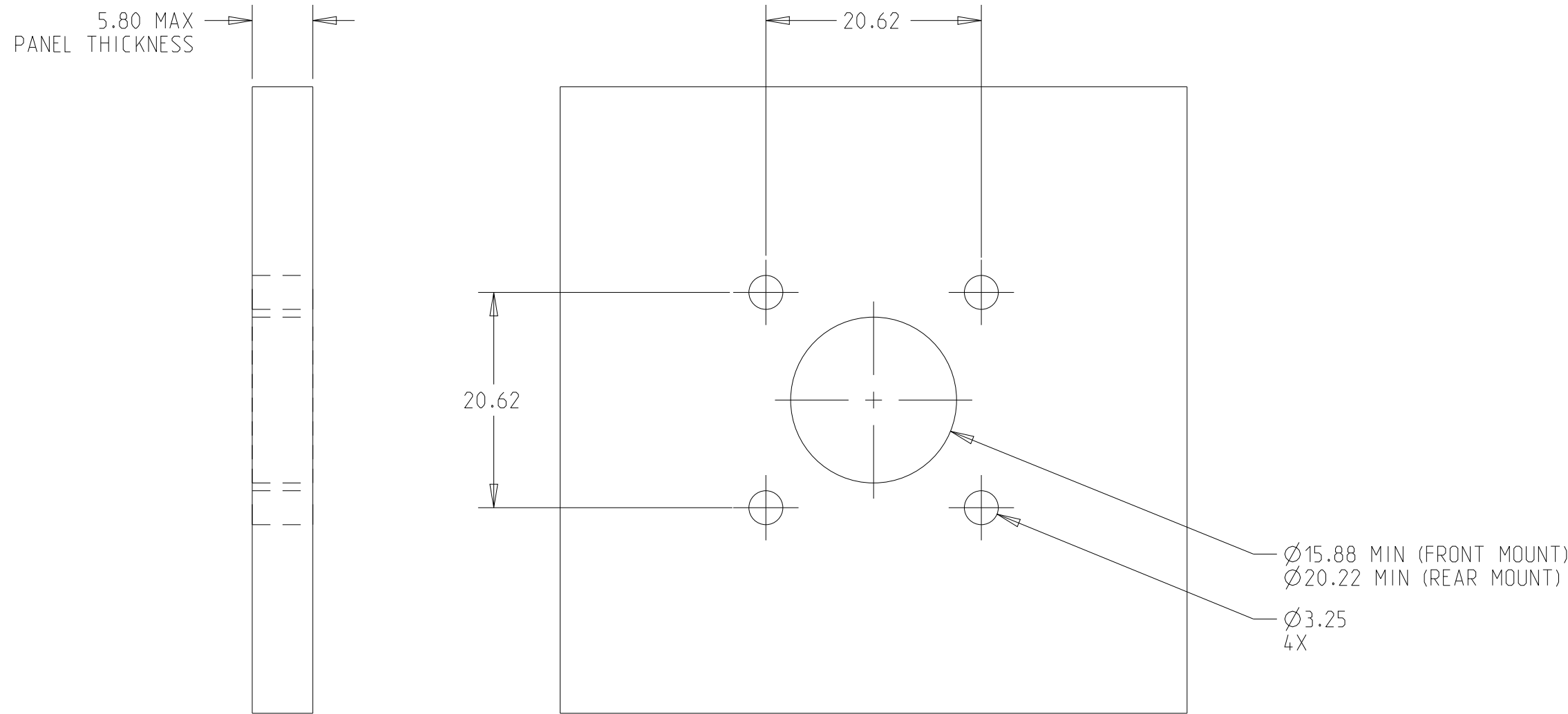
RECOMMENDED PANEL CUT-OUT SCALE 2:1
