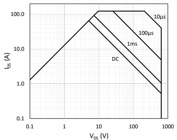
Fig. 14. Safe Operating Area, T_{CASE} = 25^{\circ}\text{C}
