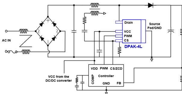
Boost PFC
