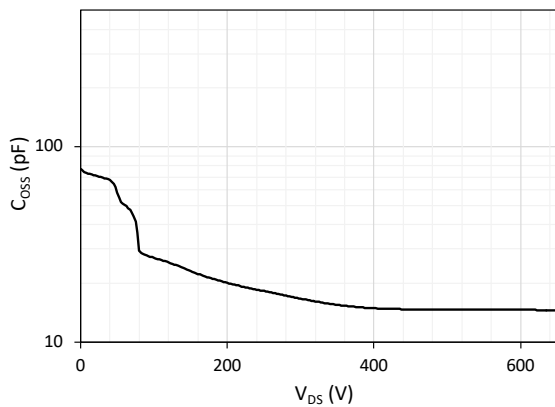
Figure 9. Output capacitance ( C_{OSS} ) vs. drain-to-source voltage ( V_{DS} )
