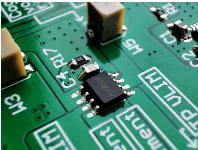
Figure 1. Physical Photos of AT8557
