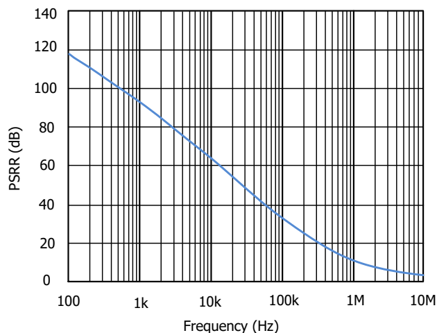
Frequency (Hz) Power-Supply Rejection Ratio vs. Frequency
