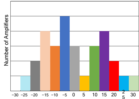
Input Offset Drift ( \text{nV}/^\circ\text{C} ) Offset Voltage Drift Production Distribution
