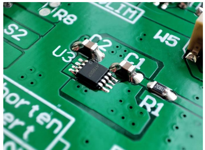
Figure 1. Physical Photos of AT8557
