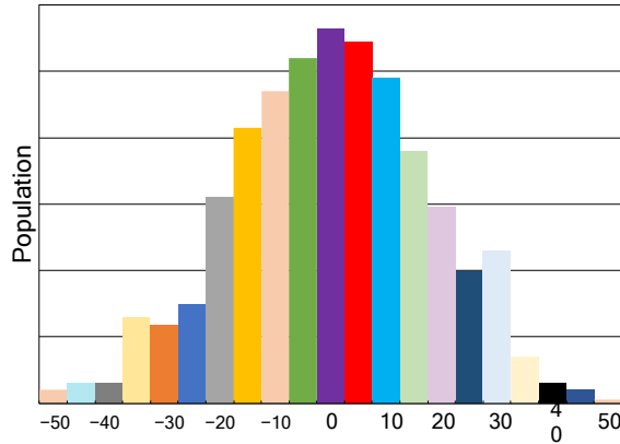
Offset Voltage ( \mu\text{V} ) Offset Voltage Production Distribution
