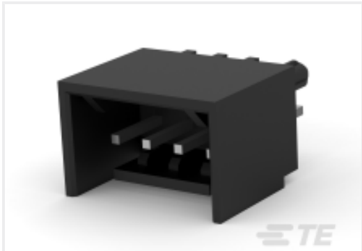
TE Part #CAT-104MTA-PVSHH Polyester Vertical PCB Header: 2.54 mm, Shrouded, MTA 100
