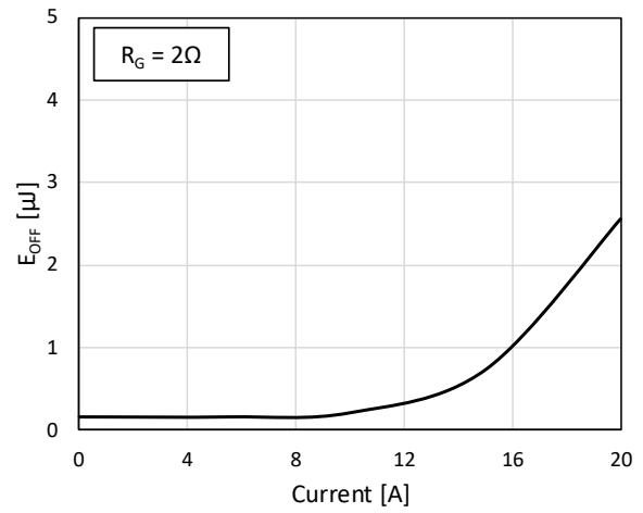
Fig. 16. E_{OFF} vs. I_{DS} , T_{JUNC} = 25\text{ °C}
