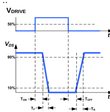
Figure 2. Prop Delay, Rise/Fall Time
