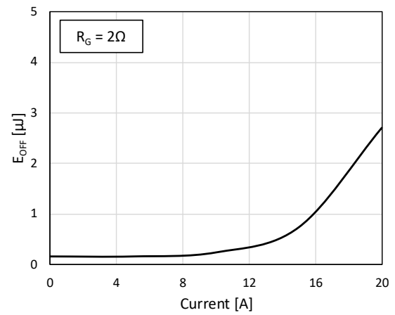
Fig. 18. E_{OFF} vs. I_{DS} , T_{JUNC} = 125\text{ °C}
