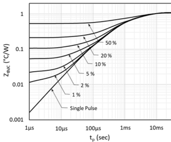
Fig. 13. Transient R_{\theta\_JUNC-CASE}
