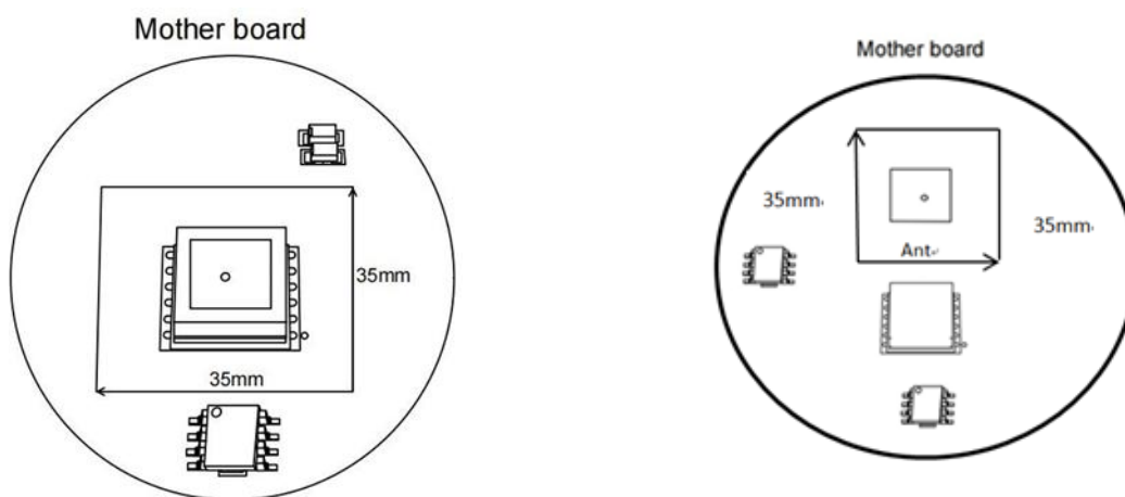
Figure 15: Recommended Ground Plane
