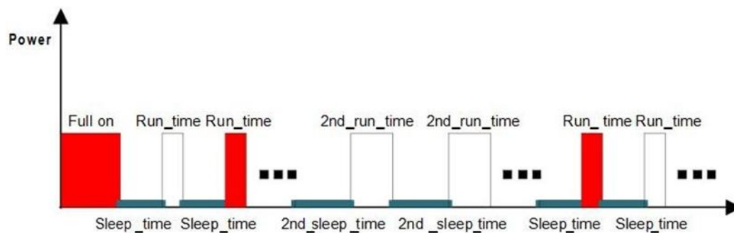
Figure 8: Periodic Mode
