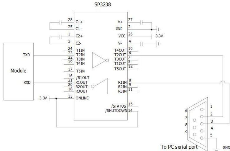
Figure 11 : RS-232 Level Shift Circuit
