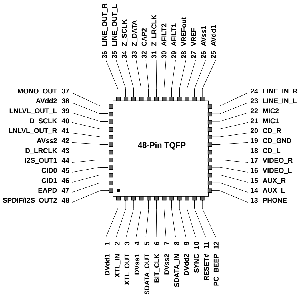
Figure 22. STAC9756/57 Pin Description Drawing
