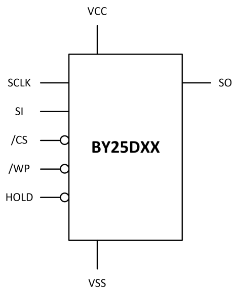
Figure 2. Pin Configuration SOP8/TSSOP8
