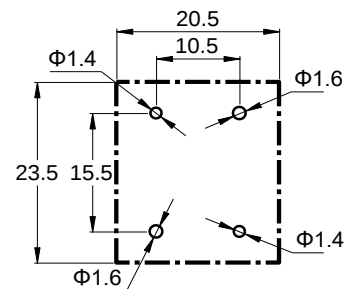
Reference Hole Pattern
