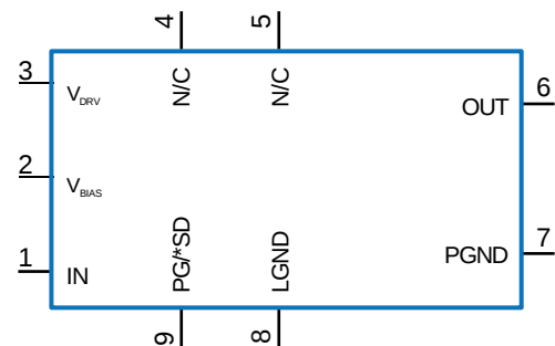
Figure 7. Suggested FBS-GAM01-P-C50 Schematic Symbol
