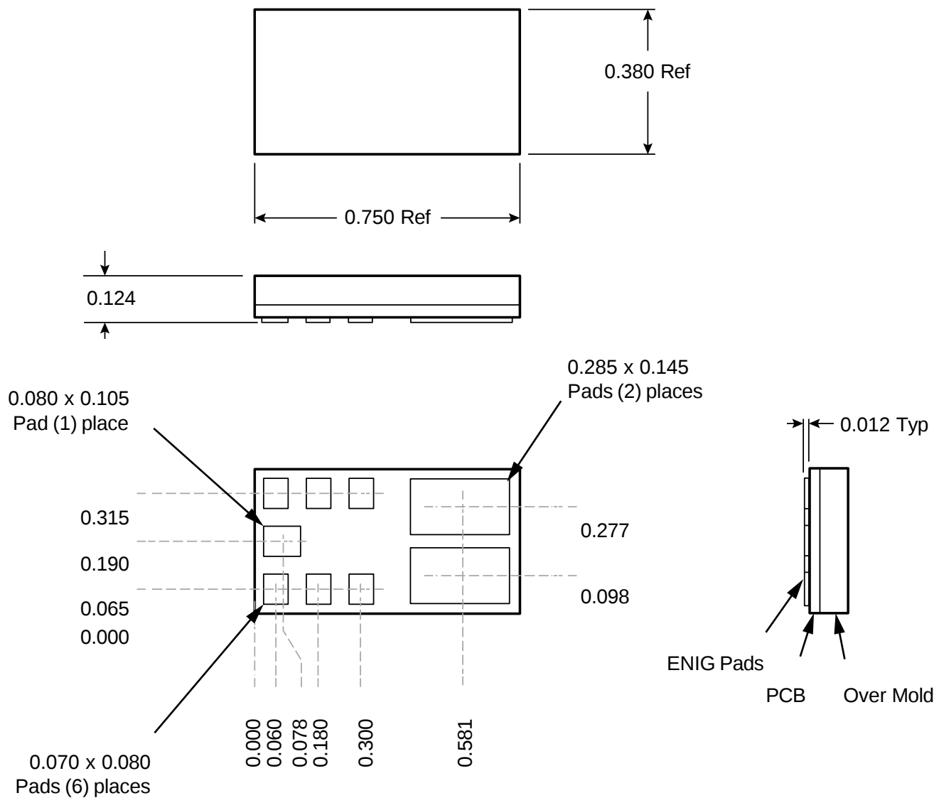
Figure 10. FBS-GAM01-P-C50 Package Outline and Dimensions
