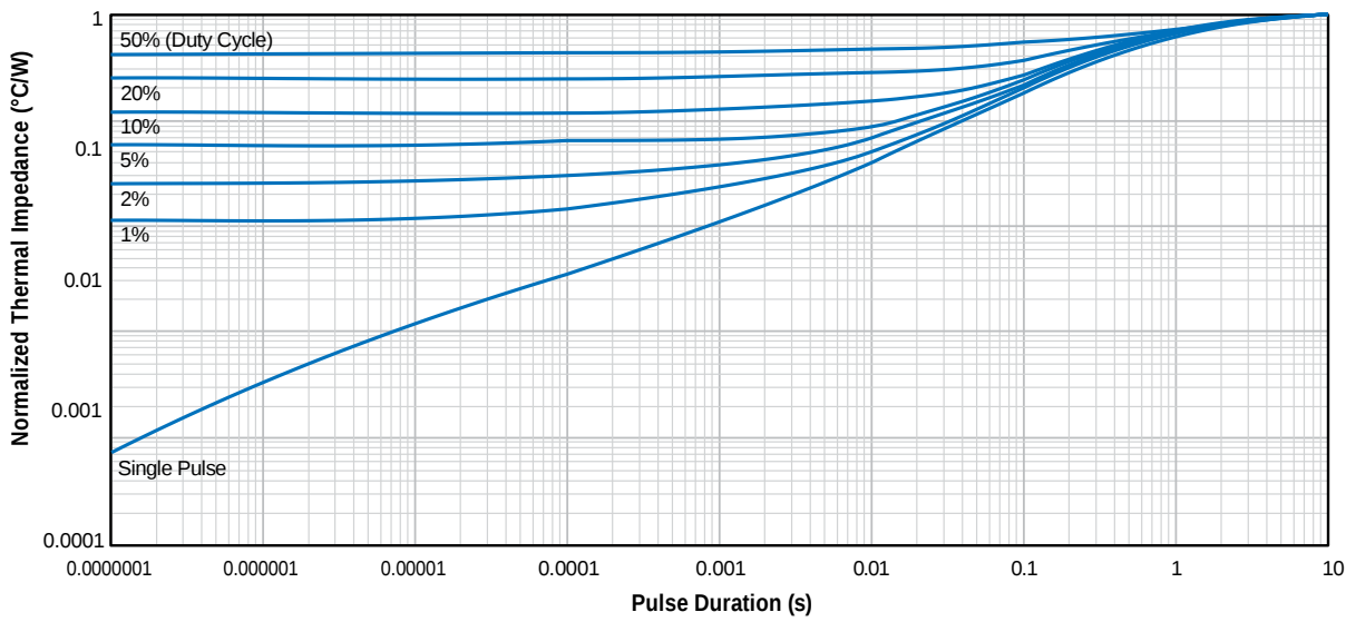
Figure 7. Typical Catch Schottky Normalized Junction-to-Case Thermal Impedance
