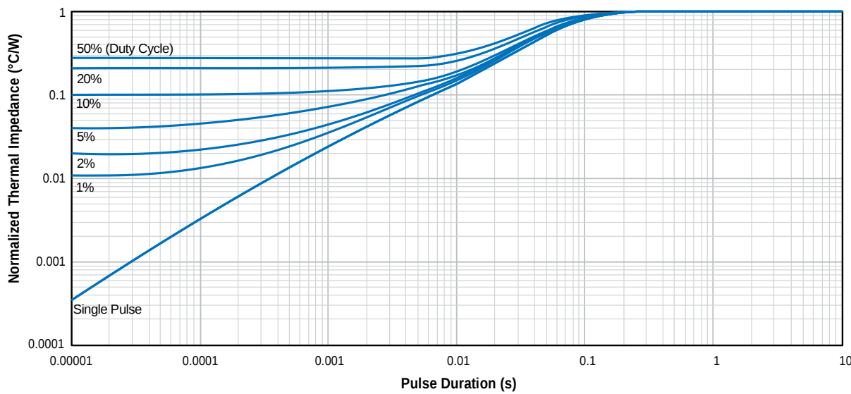
Figure 8. Typical Power eGAN® HEMT Normalized Junction-to-Case Thermal Impedance
