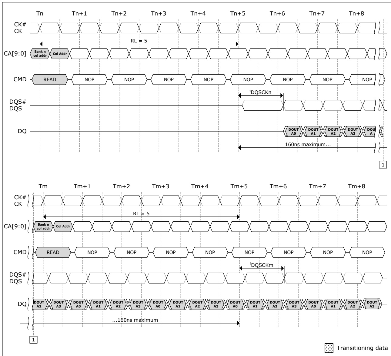
Figure 4.10 - t_{DQSKDS} timing
