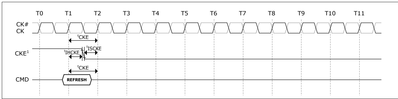
Figure 4.51 - Refresh command to power-down entry
