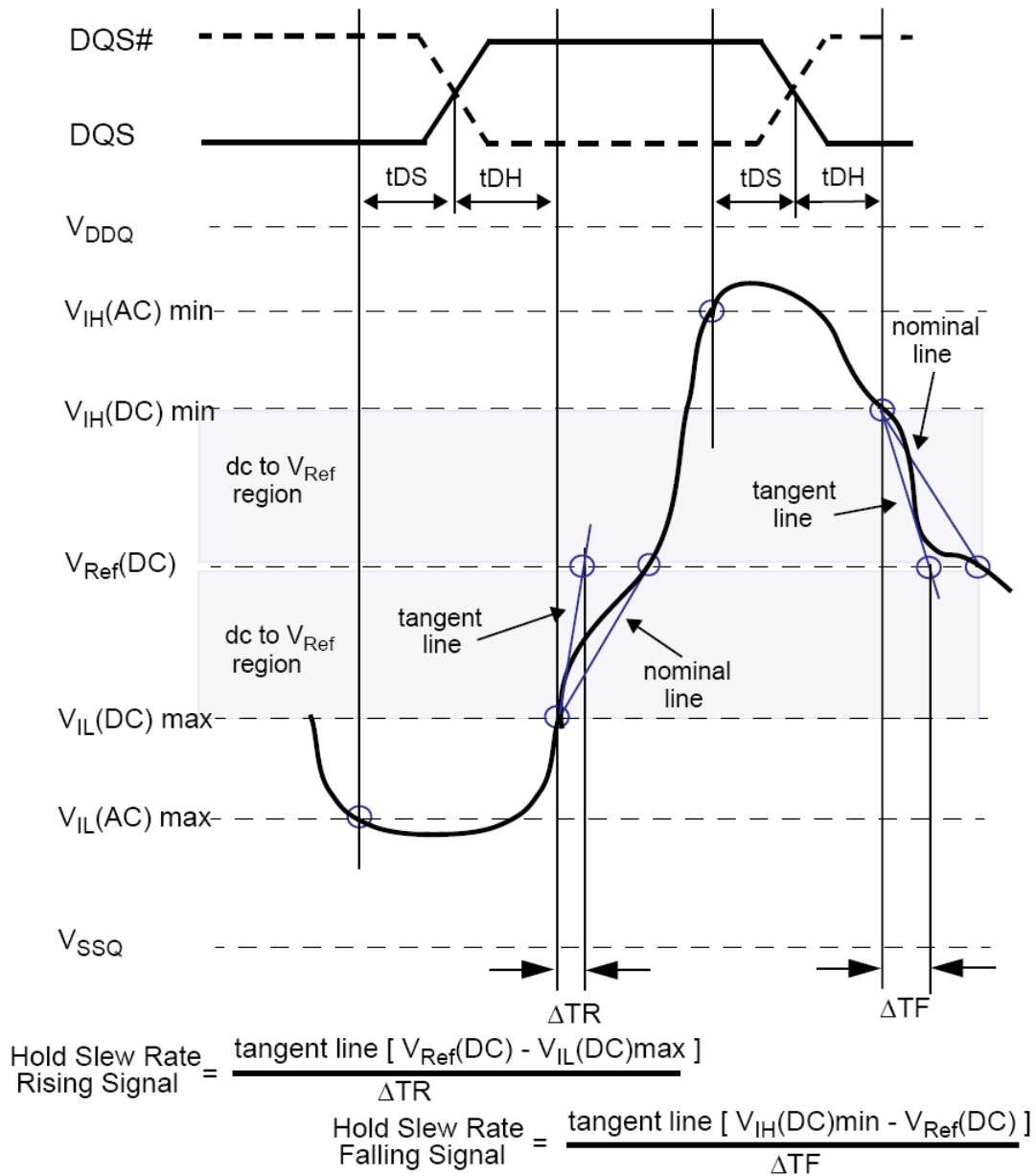
Figure 11.9 - Illustration of tangent line for for hold time tDH for DQ with respect to strobe
