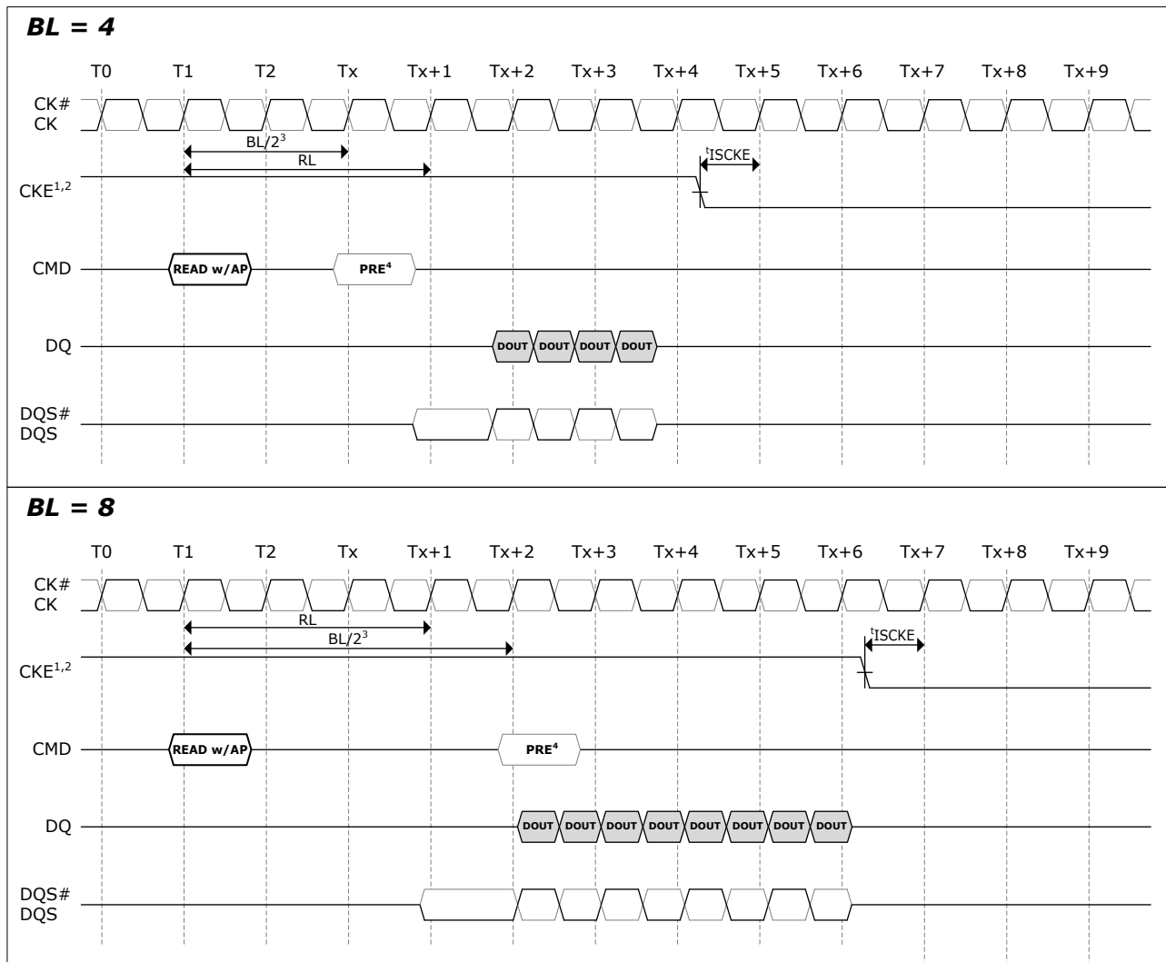
Figure 4.48 - Read with autoprecharge to power-down entry
