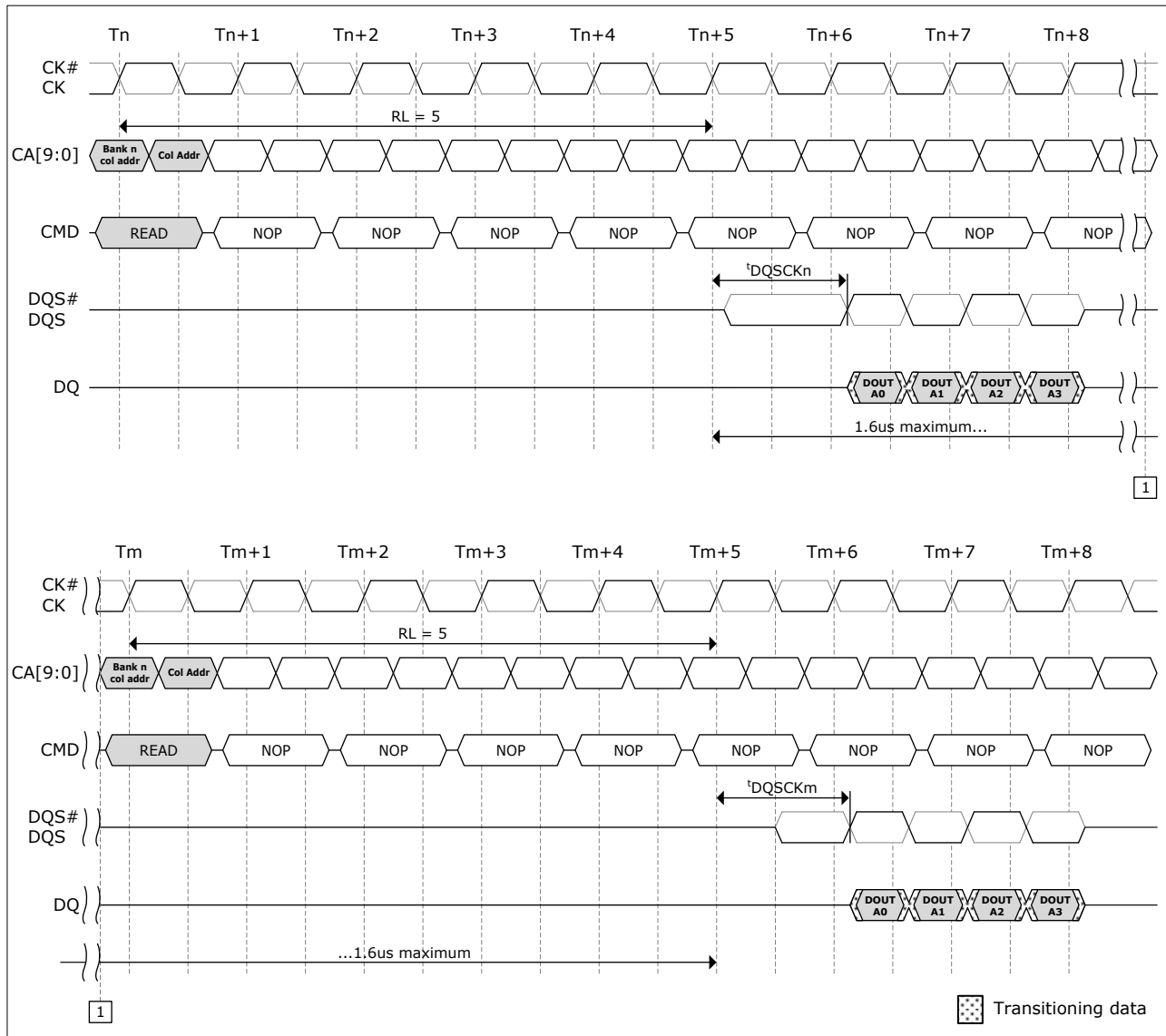
Figure 4.9 - t_{DQSKDM} timing
