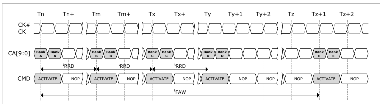
Figure 4.2 - t_{FAW} timing
