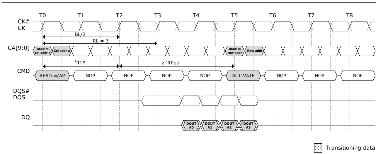
Figure 4.24 - Burst read with Auto-Precharge: RL = 3, BL = 4, RU(tRTP(min)/tck) = 2
