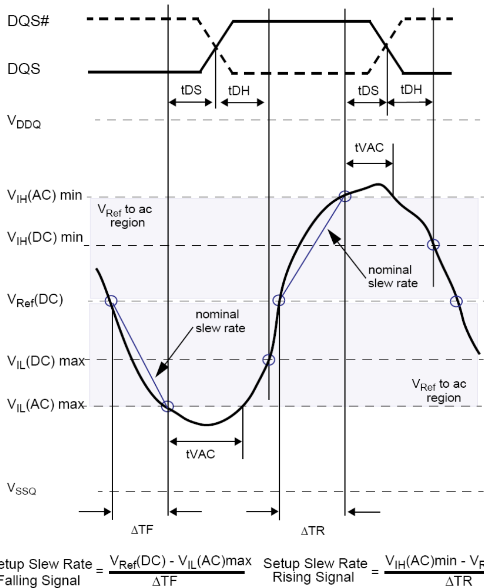
Figure 11.6 - Illustration of nominal slew rate and tVAC for setup time tDS for DQ with respect to strobe
