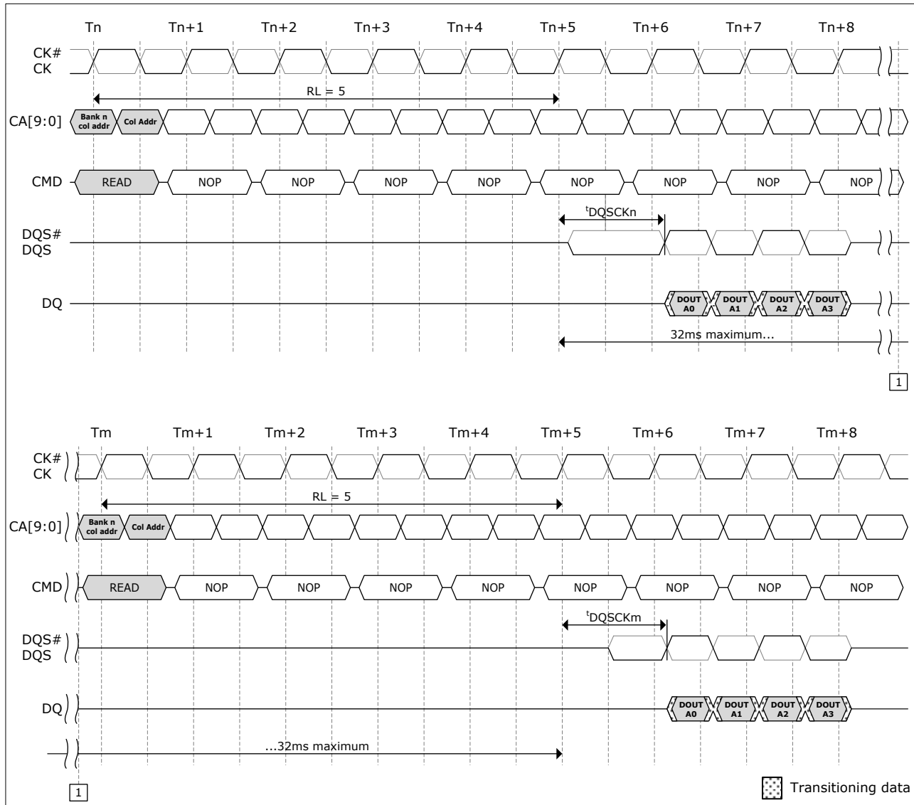
Figure 4.8 - t_{DQCKDL} timing
