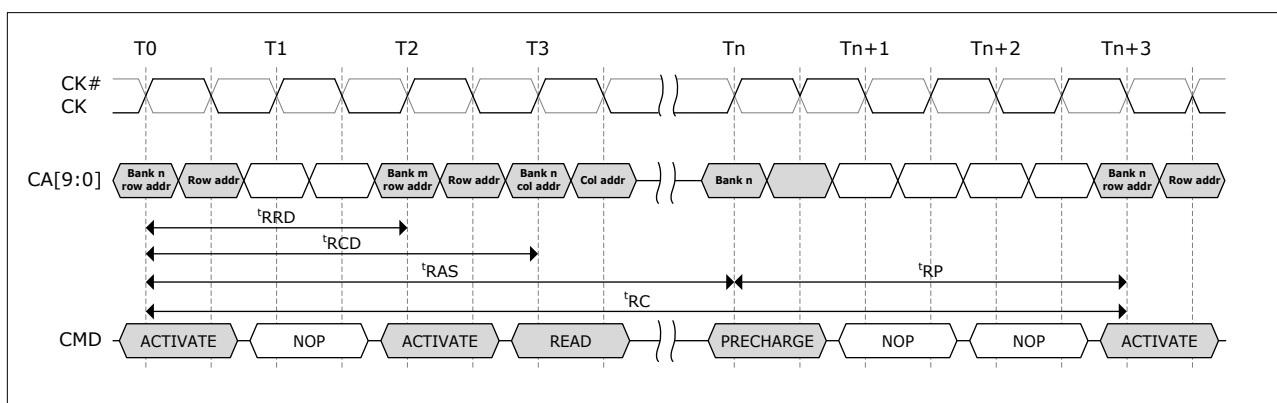
Figure 4.1 - Activate command cycle: t_{RCD} = 3 , t_{RP} = 3 , t_{RRD} = 2
