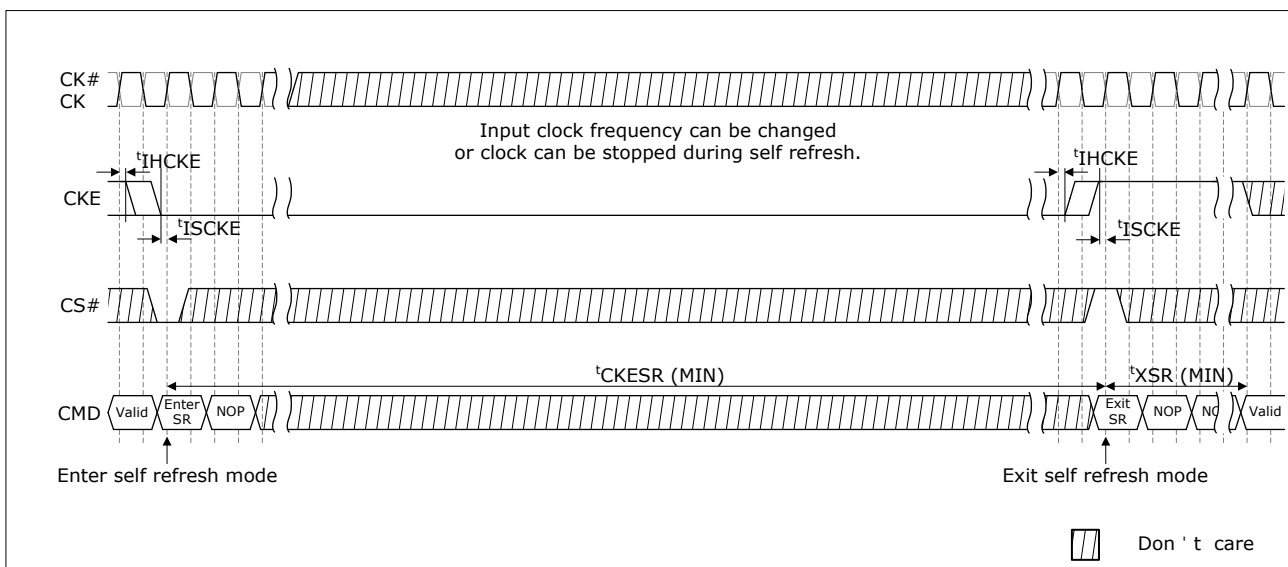
Figure 4.33 - Self-Refresh Operation
