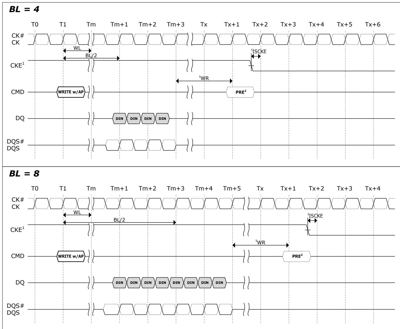
Figure 4.50 - Write with autoprecharge to power-down entry
