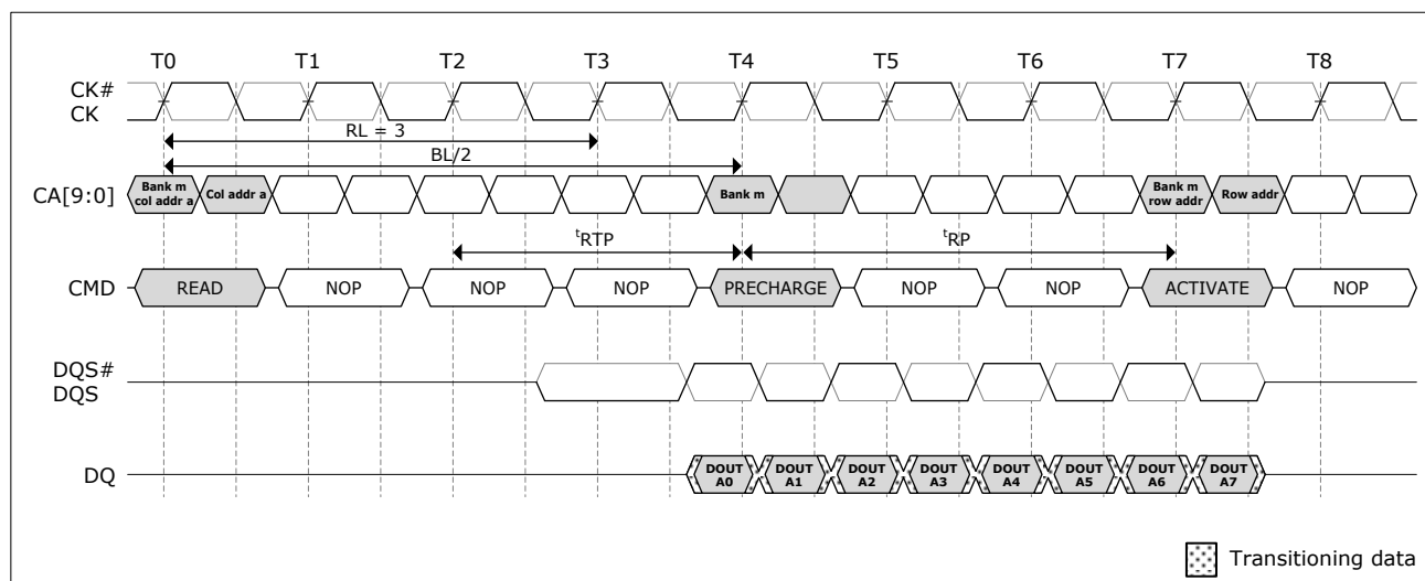
Figure 4.21 - Burst read followed by Precharge: RL = 3, BL = 8, RU(tRTP(min)/tCK) = 2
