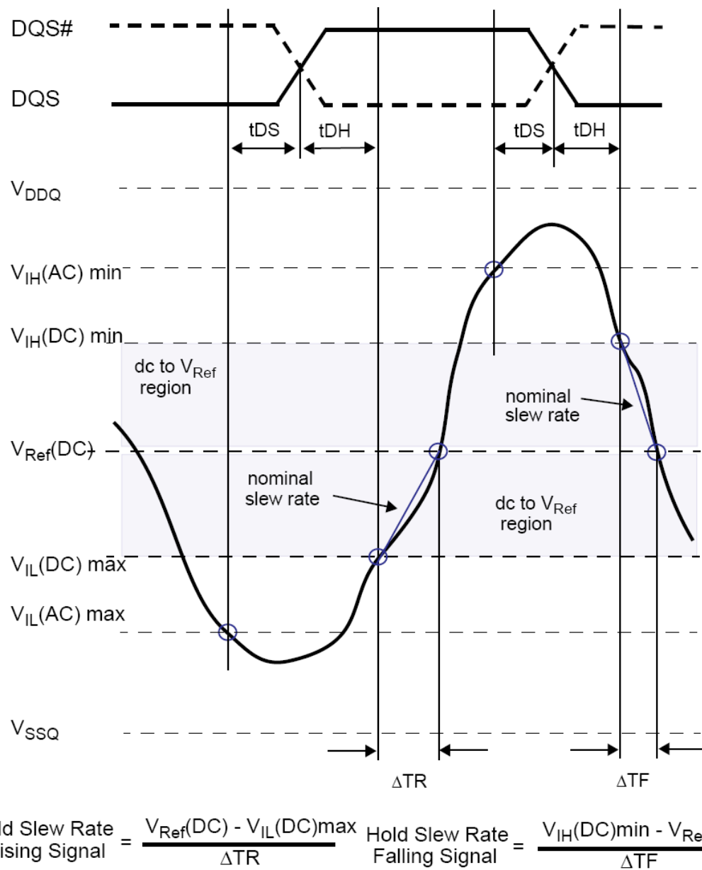
Figure 11.7 - Illustration of nominal slew rate for hold time t_{DH} for DQ with respect to strobe
