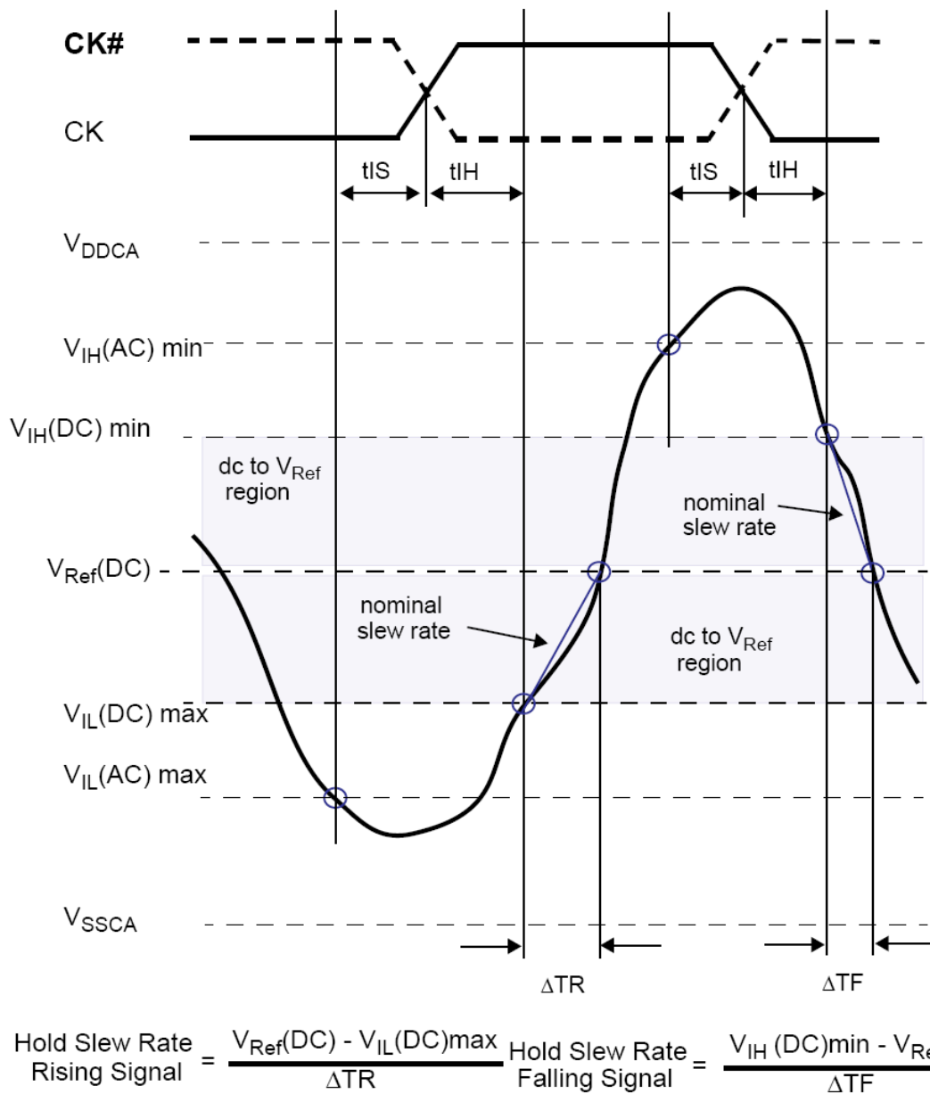
Figure 11.3 - Illustration of nominal slew rate for hold time t_{IH} for CA and CS# with respect to clock
